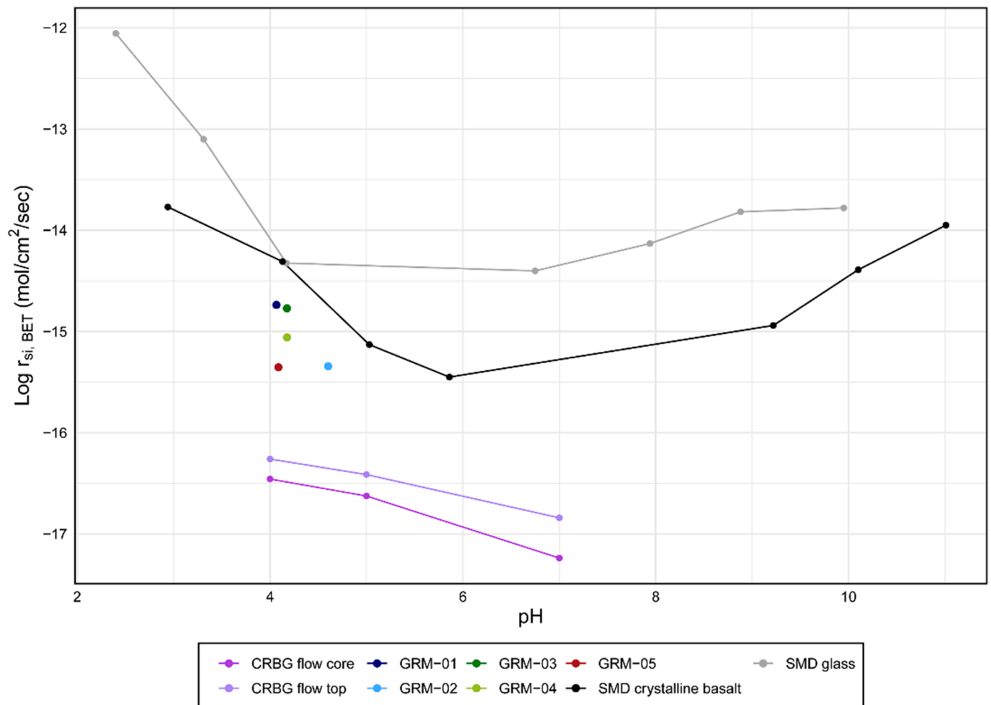
Fig. 10. Comparison between the steady-state dissolution rates of the five field samples from this study and the experimental results of Schaef and McGrail (2009) and Gudbrandsson et al. (2011) at 25 °C. Stapafell Mountain Dyke in Iceland (SMD). Columbia River Basalt Group (CRBG) in the US.
