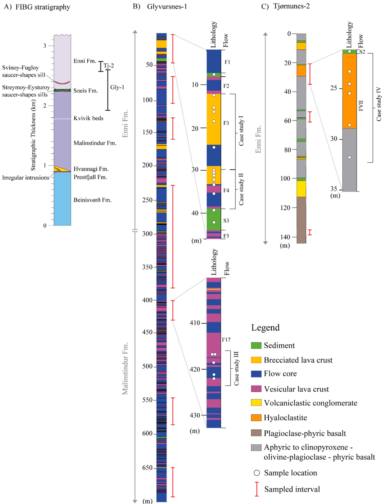
Fig. 2. Overview of boreholes used in this study. A) Stratigraphic locations of the Tjørnunes-2 (Tj-2) and Glyvursnes-1 (Glyv-1) boreholes (modified from Passey and Jolley, 2009 ). B) Lithological log of the Glyvursnes-1 borehole with sample locations indicated (modified from Waagstein, 2002a ). C) Lithological log of the Tjørnunes-2 borehole with sample locations indicated (modified from Jolley and Passey, 2012 ). Case study intervals are marked.
