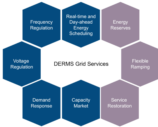
Fig. 12. Grid services supported by DERMS – Flexible load compatible (in blue) and PV/BESS compatible (in beige).
