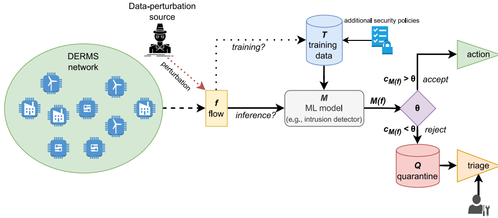
Fig. 11. Data-perturbation scenario and a potential defense. We consider adversarial perturbations that can “poison” (i.e., negatively affect) the output of the ML model either during its training stage (i.e., when such perturbations are put in the training data) or during its inference stage (i.e., when the perturbations only entail samples analysed by the model during its operational phase). An exemplary use-case is an ML model for intrusion detection.
