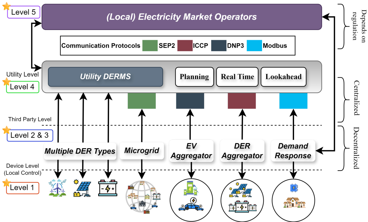
Fig. 5. Hybrid DERMS. In addition to the flexibility (i.e., DER scalability, communication) this architecture supports, the integration of centralized and decentralized operation provides broader functionalities (e.g., management and optimization of DERs) across multiple levels [17].
