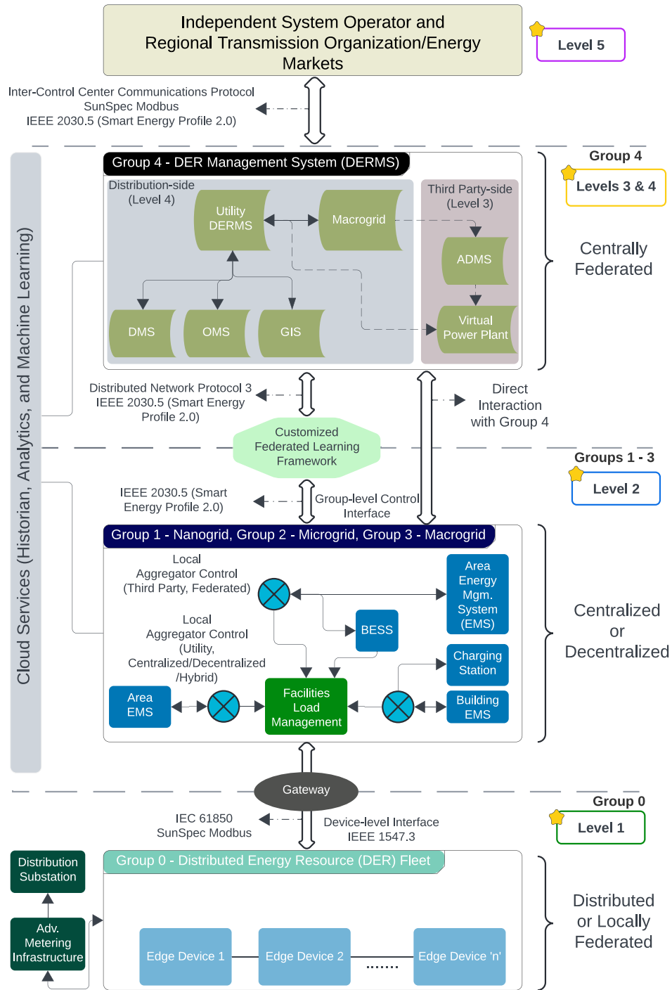
Fig. 2. Hierarchical Hybrid DERMS Federated Learning framework. Each level starting from Level 1 (bottom-most) to Level 5 (top-most) interacts with other levels through multiple protocols (e.g., Modbus, SEP) and accommodates different DERMS architecture types based on the factors unique to each architecture type.
