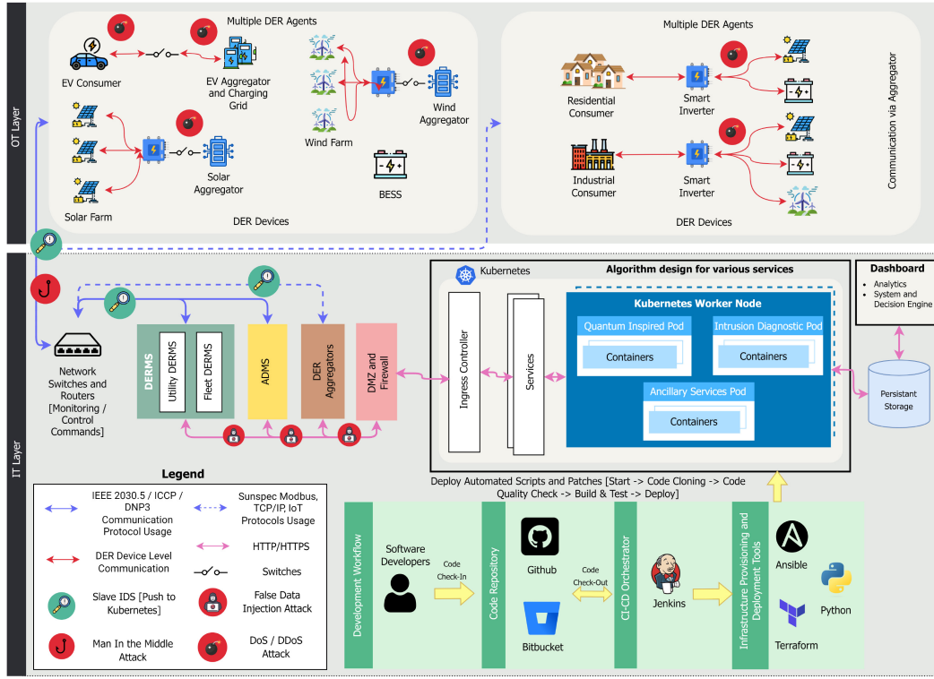
Fig. 8. Integrated AI-ready DERMS Edge Testbed at the University of North Dakota. Interactions between the IT and OT layers warrants a flexible and scalable framework that can support large deployments across any region (i.e., through Kubernetes), cater to lightweight edge computing hardware, and anticipate common cyber threats (e.g., DoS, MiTM) at each layer.
