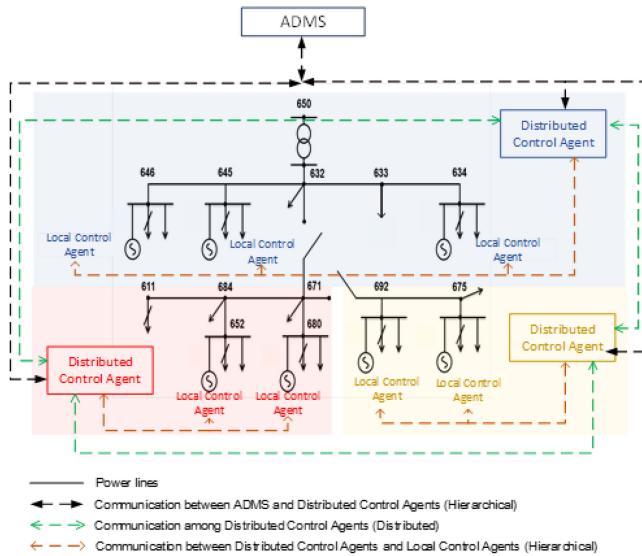
Fig. 13. Layered architecture mapped for distributed applications.
