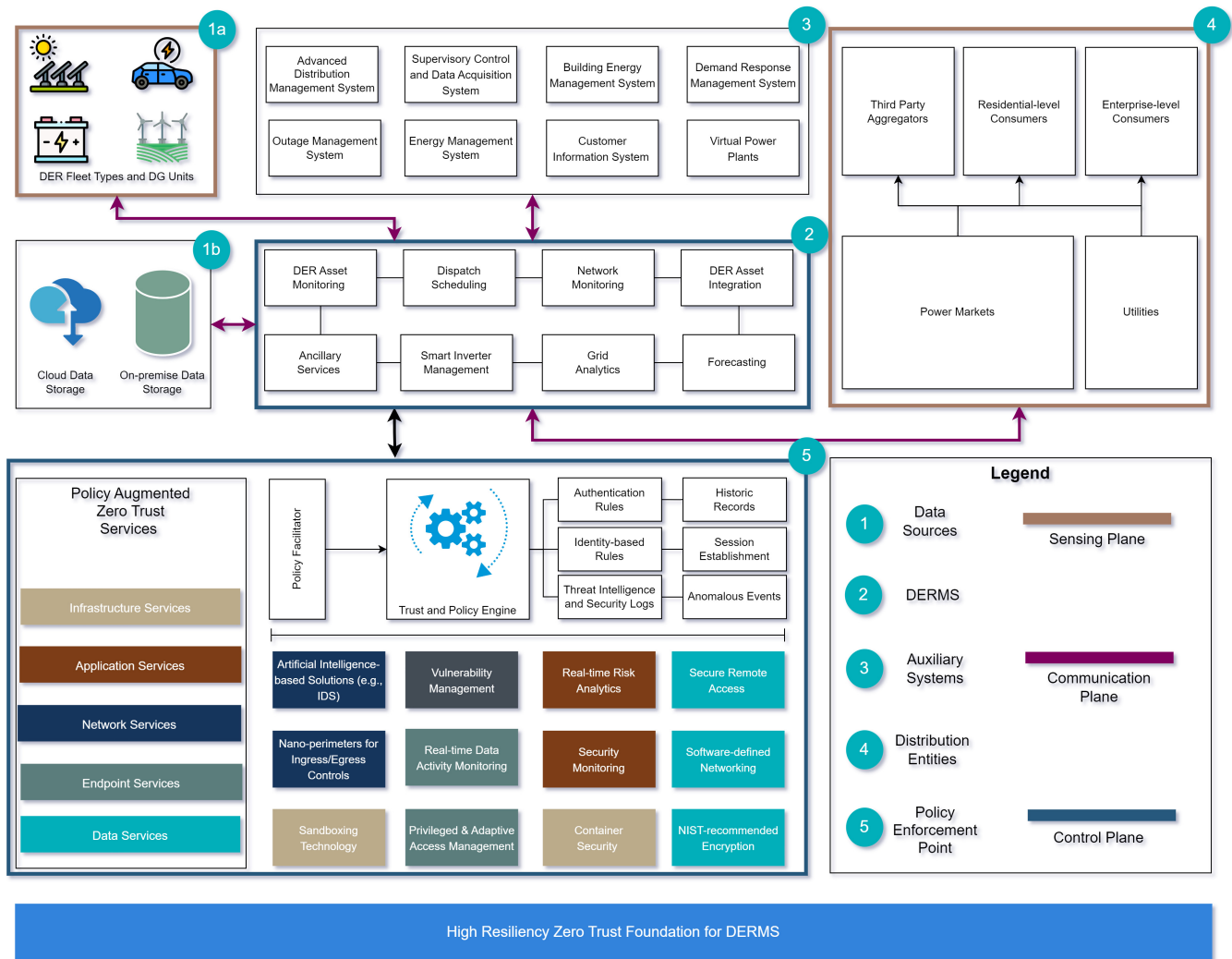
Fig. 10. High resiliency zero trust foundation for DERMS. We identify multiple data sources (e.g., DER fleets, data-at-rest in cloud), distribution entities (e.g., power markets), and the role of DERMS in managing the communication and control planes. Zero trust entities (e.g., policy engine) are implemented in the back-end and can render different service types (e.g., data, application) based on need.
