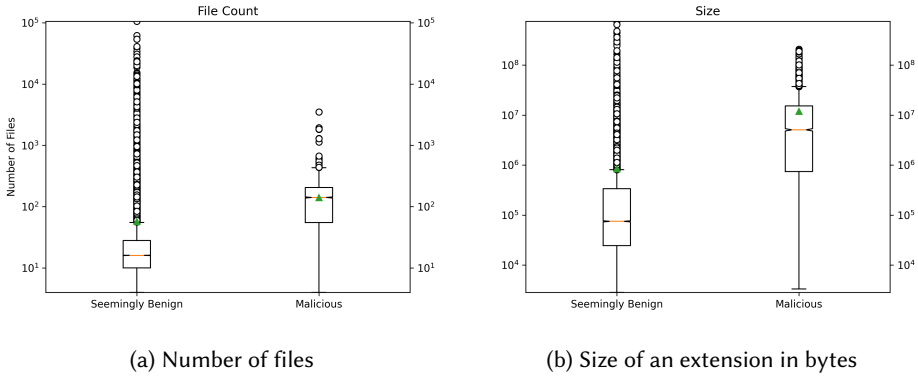
Fig. 6. Distribution of two features for benign and malicious extensions.
