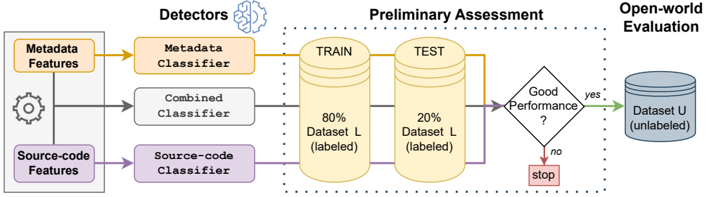
Fig. 3. Workflow: if our detectors exhibit good performance on Dataset L, we use them on Dataset U.
