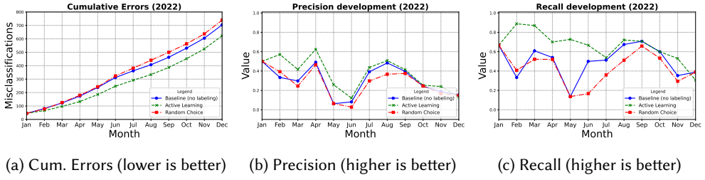
Fig. 8. Experiments with active learning. The blue line corresponds to the Combined classifier trained on all extensions before Jan 1st 2022 (and never re-trained). The green line corresponds to the Combined classifier that is re-trained monthly on an extra 15 extensions for which the model was “the most uncertain” the previous month. The red line corresponds to the Combined classifier that is monthly re-trained by including an extra 15 randomly chosen extensions of the previous month.
