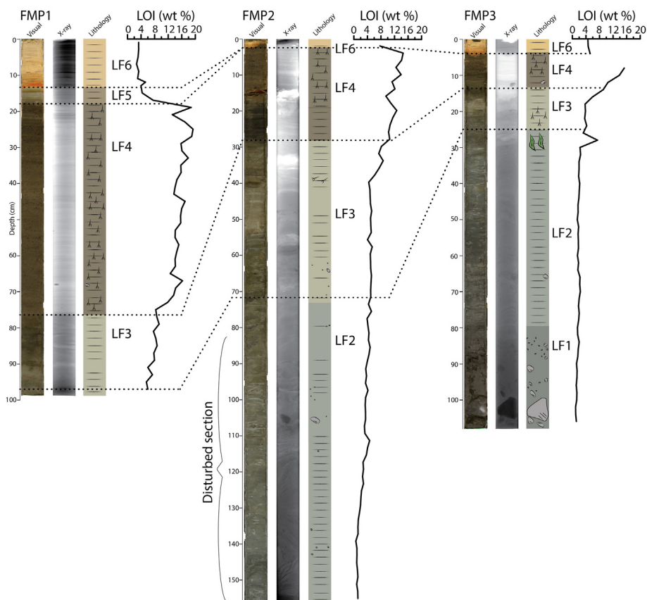
Fig. 7. Correlation of the three sediment cores FMP1, FMP2 and FMP3. Core photograph, X-ray image, lithological log and LOI. For legend see Fig. 6c.
