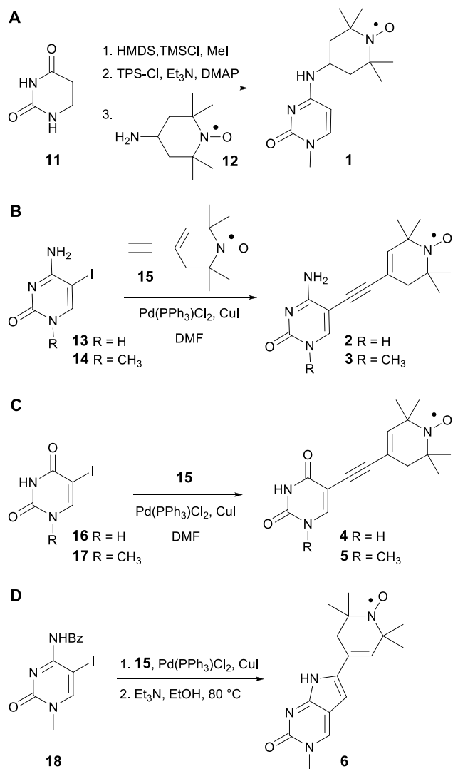
Scheme 1: Synthesis of 4-amino- ( A ), acetylene- ( B and C ), and pyrrolo- ( D ) linked pyrimidine spin labels. Bz = benzoyl.
