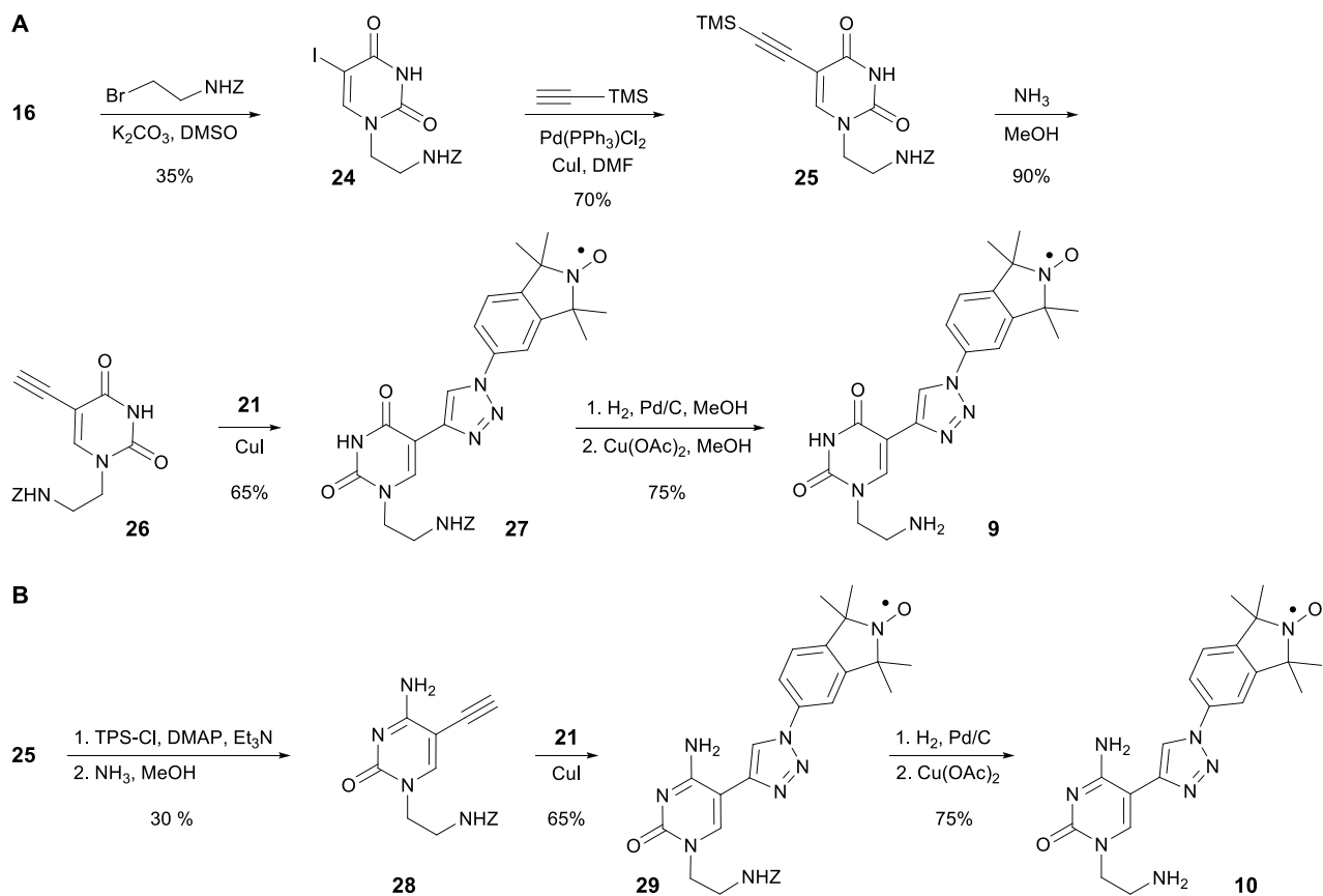
Scheme 3: Synthesis of N1-ethylamino triazole-linked spin labels 9 and 10 . Z = carboxybenzyl.
