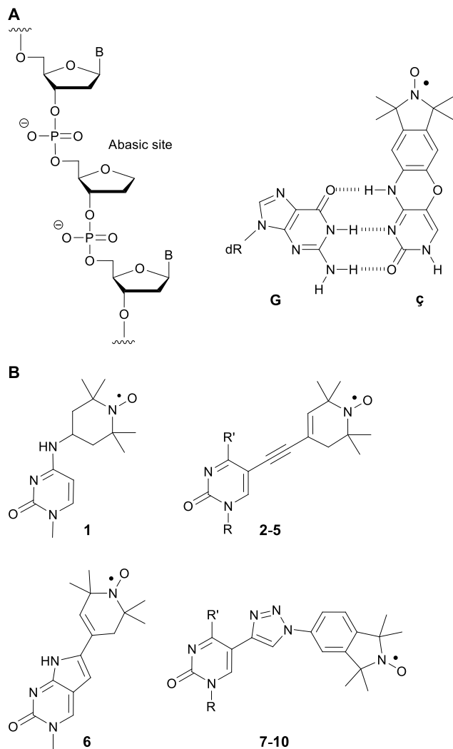
Figure 1 A. Left. Structure of an abasic site. Right. Structure and base pairing scheme of the spin label \zeta with guanine (G). dR = deoxyribose. B. Structures of pyrimidine-derived spin labels prepared in this study. R = -H, -CH 3 or -CH 2 CH 2 NH 2 and R' = -OH, -NH 2 .
