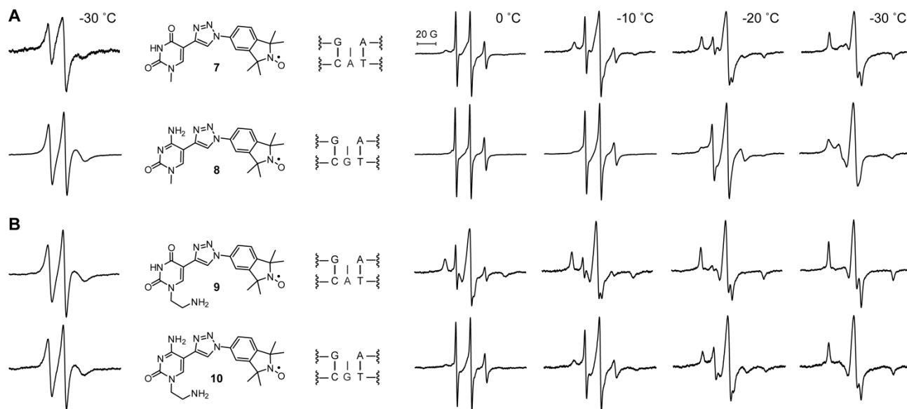
Figure 3: EPR spectra of triazole-linked N1-methyl ( A ) and N1-ethylamino ( B ) spin labels (left) and in the presence of duplex DNA containing an abasic site (right). For clarity, only a part of the DNA construct is shown. The complete DNA sequence is 5'-d(GAC CTC G_A TCG TG)-3' and its complementary strand 5'-d(CAC GAT XCG AGG TC)-3', where _ is an abasic site and X is the orphan base opposite the abasic site.
