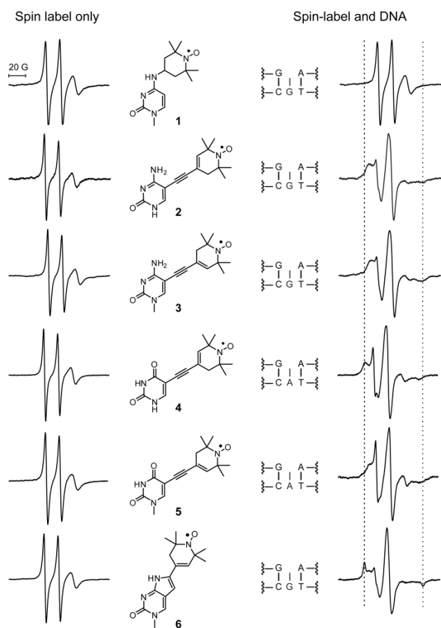
Figure 2: EPR spectra of spin labels (left) and in the presence of an abasic site containing DNA duplex at -30\text{ }^{\circ}\text{C} (right). Dotted lines indicate the relative broadening of the EPR spectra of spin labels. For clarity, only a part of the DNA construct is shown. The complete DNA sequence is 5'-d(GAC CTC G_A TCG TG)-3' and its complementary strand 5'-d(CAC GAT XCG AGG TC)-3', where _ is an abasic site and X is an orphan base opposite the abasic site.
