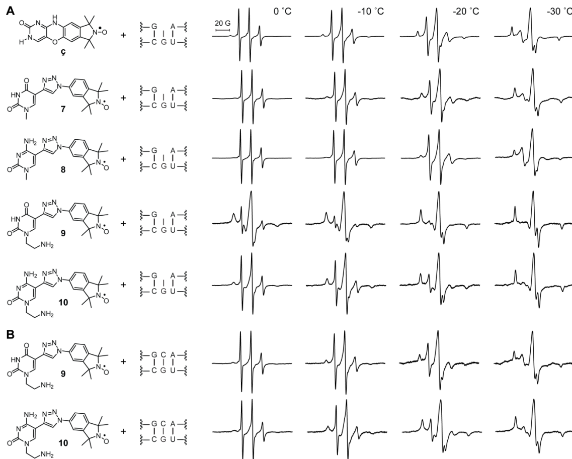
Figure 4: EPR spectra of triazole-linked spin labels in the presence of both an RNA duplex containing an abasic site ( A ) and an unmodified RNA duplex ( B ). For clarity, only a part of the RNA construct is shown. The complete RNA sequences are 5'-GAC CUC G_A UCG UG-3' and 5'-CAC GAU GCG AGG UC-3', where _ is an abasic site.
