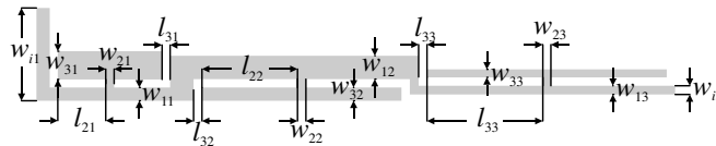
Fig. 2. Geometry of a compact UWB impedance transformer (Kurgan, Bekasiewicz and Kitlinski, 2015).
