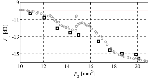
Fig. 3. The low- ( \circ ) and high-fidelity ( \square ) designs obtained using sequential domain patching.
