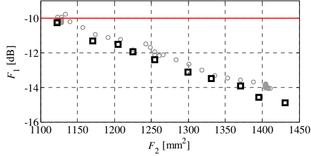
Fig. 7. The low- (○) and high-fidelity (□) designs obtained using sequential domain patching.
