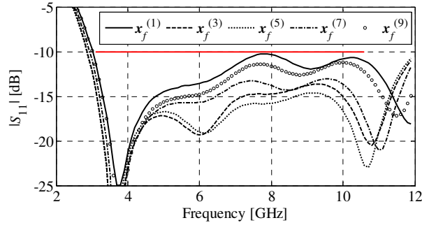
Fig. 8. Frequency characteristics of transformer designs of Table 2.
