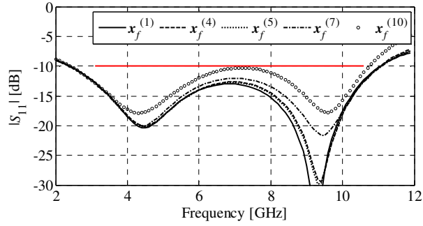
Fig. 4. Frequency characteristics of the transformer designs of Table 1.
