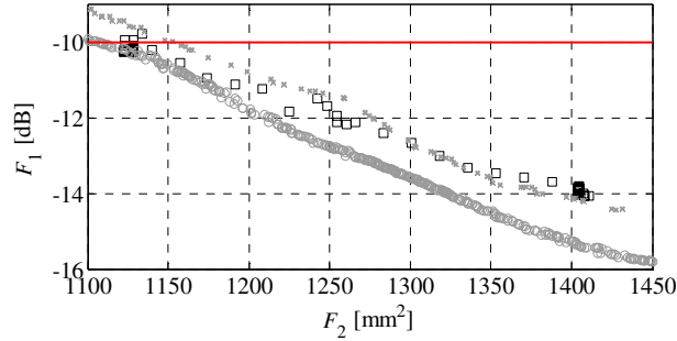
Fig. 9. Comparison of initial Pareto fronts obtained using SDP (□), as well as first (○) and second (×) benchmark method.
