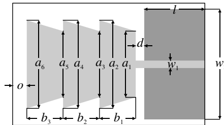
Fig. 6. Geometry of the considered monopole antenna (Koziel, Bekasiewicz and Zieniutycz, 2014).
