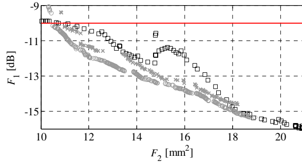
Fig. 5. Comparison of initial Pareto fronts obtained using SDP ( \circ ), as well as first ( \square ) and second ( \times ) benchmark method.
