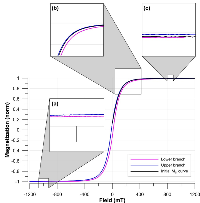
Figure 5. Hysteresis measurement of a sample from core section 9-02 (section depth: 79–80 cm) corresponding to a core depth and core age of 15.83–15.84 m and about 20.6 ka. Inset (a) The upper and lower branch of the hysteresis remaining slightly open in fields of 1 T. Inset (b) The ratio of the areas enclosed by the hysteresis branches and the M_{SI} curve. Inset (c) The gap between the upper and lower branches of the hysteresis loop, causing the ratio of E_L^A/E_{hys} to be indeterminate.
