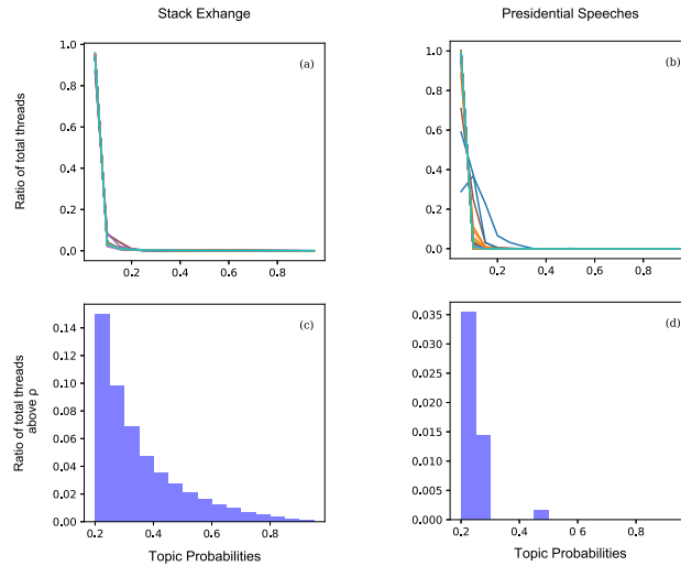
Fig. 3. Calibration of the minimum relevance ( \rho )—[Top] Probability distributions for the topics ( n = 50 , each line is a topic) in each thread, with \rho = 0.2 . [Bottom] Validation of our selection: for Speeches (StackEx), few (many) threads are > \rho .
