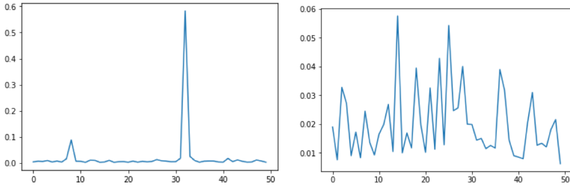
Fig. C1. Validation of our heuristic —We plot the relevance ( y -axis) for the 50 chosen topics on StackEx and Speeches.
