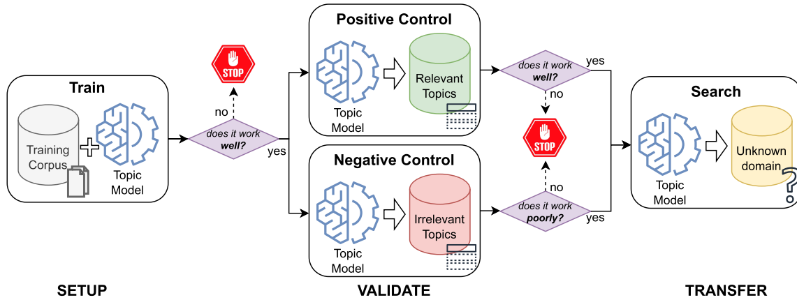
Fig. 1. Schematic description of the TOPTRAN protocol. The conventional topic modeling is built based on the training corpus from a known domain and validated on two other corpora from a related and an unrelated domain. Subsequently, the model can be “transferred” for searching for topics from a known domain in the unknown one.
