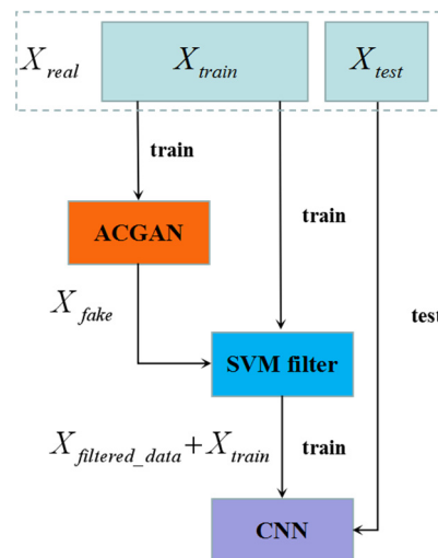
Figure 4. ACGAN-SVM-CNN.
