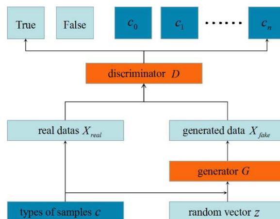
Figure 1. Main Structure of ACGAN.
