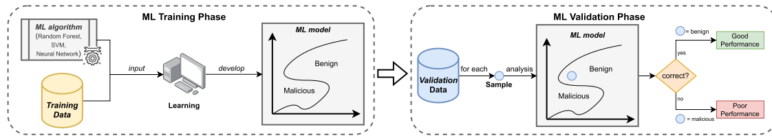
Fig. 1. Machine Learning development. After collecting some training data and analyzing such data via an ML algorithm, an ML model is obtained. Such an ML model must be tested via some validation data. If the performance of such an assessment is appreciable, then the ML model can be deployed in production.
