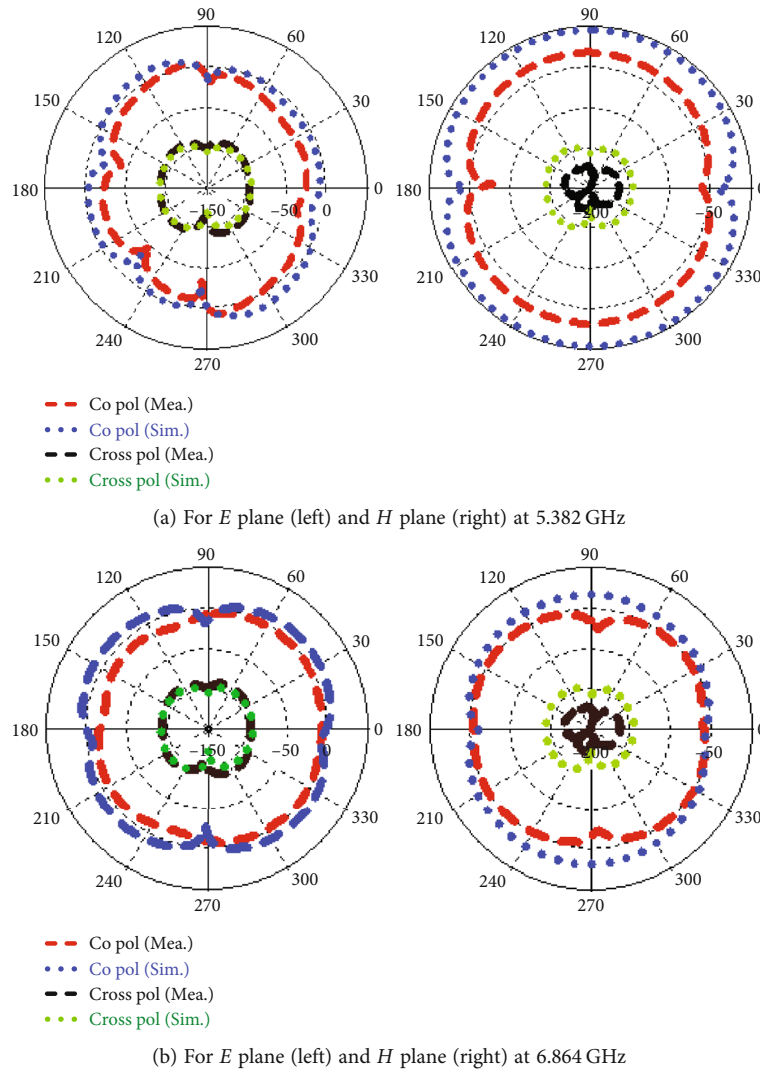
FIGURE 8: Measured and simulated copolarization and cross-polarization.
