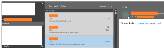
(a) Aside from the “benign” email (sent at 15:19), the two “quishing” emails (one having the QR code as attachment, the other embedded in the email’s content) were not put in the junk folder—thereby evading the phishing/spam detection filter.
