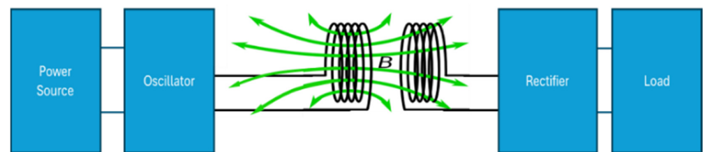
Figure 12. Schematic circuit diagram of contactless power transmission using inductive coupling for a charging system.
