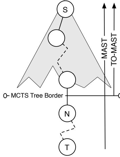
Figure 4.1: Difference between back-propagation activity of MAST and TO-MAST
