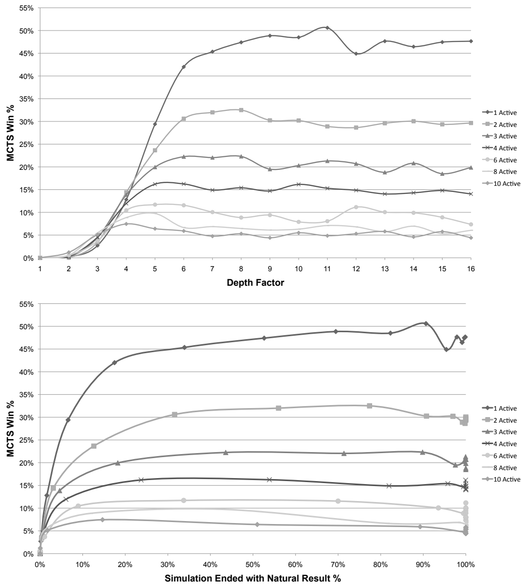
Figure 7.6: Progression Depth Factor: Fixed simulation count
