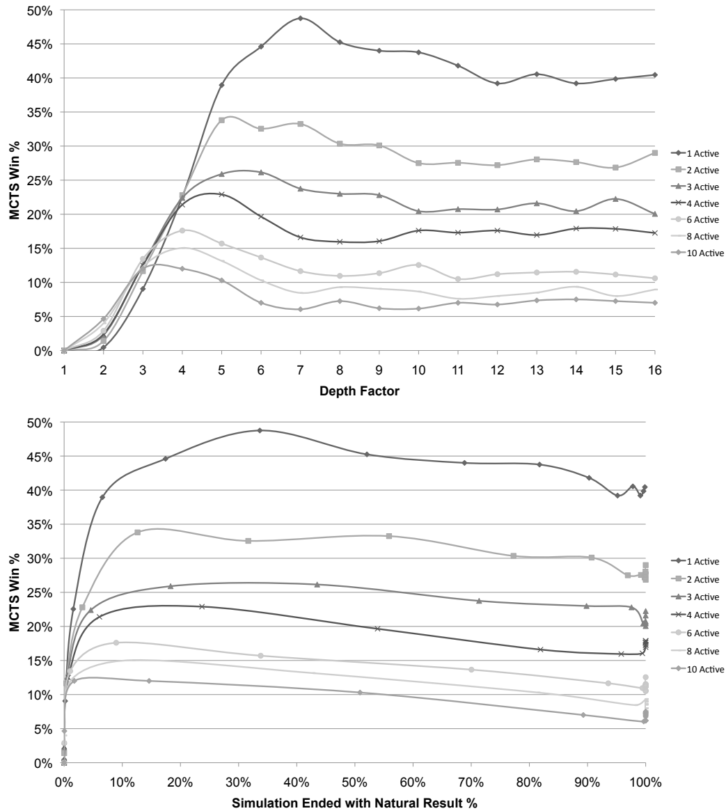
Figure 7.5: Progression Depth Factor: Fixed node expansion count
