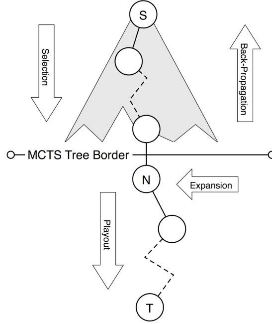
Figure 2.2: An overview of a single simulation
