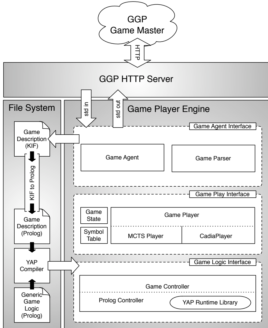
Figure 3.1: Overview of the architecture of CADIPLAYER
