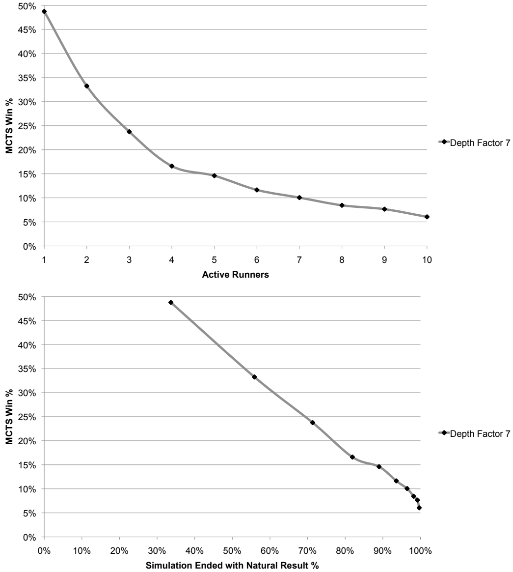
Figure 7.7: Progression Active Runners: Fixed node expansion count
