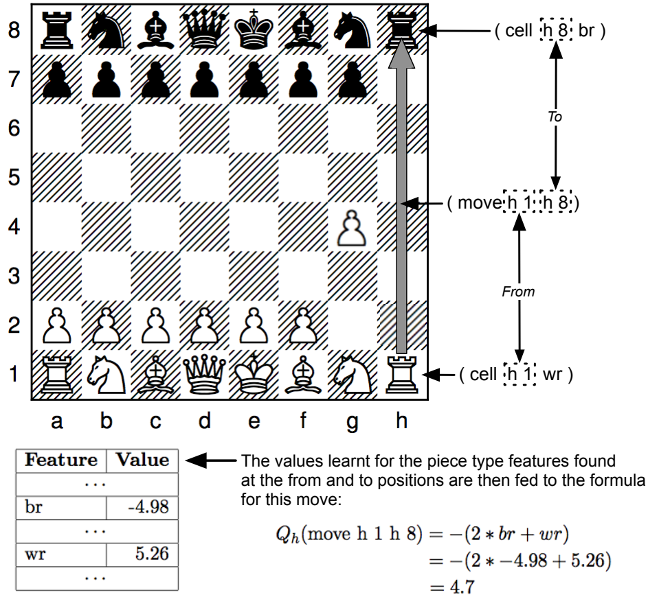
Figure 4.2: FAST capture calculations in Chess for (move h 1 h 8) in a state containing (cell h 1 wr) and (cell h 8 br) .
