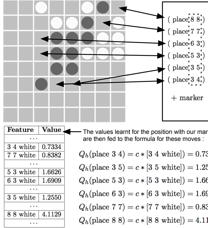
Figure 4.3: FAST calculations in Othello for available moves.
