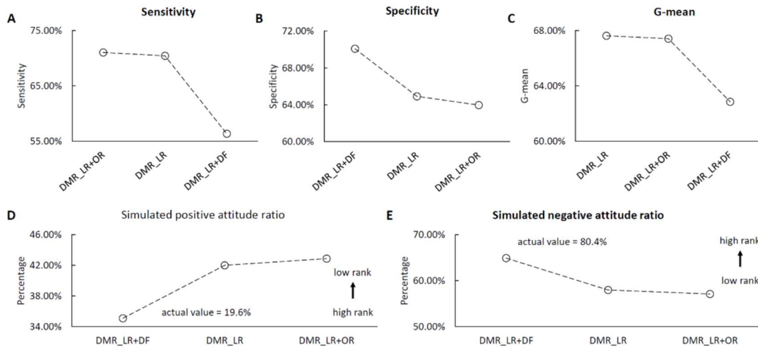
FIG. 3. Performance comparison: DMR_LR, DMR_LR+DF and DMR_LR+OR.
