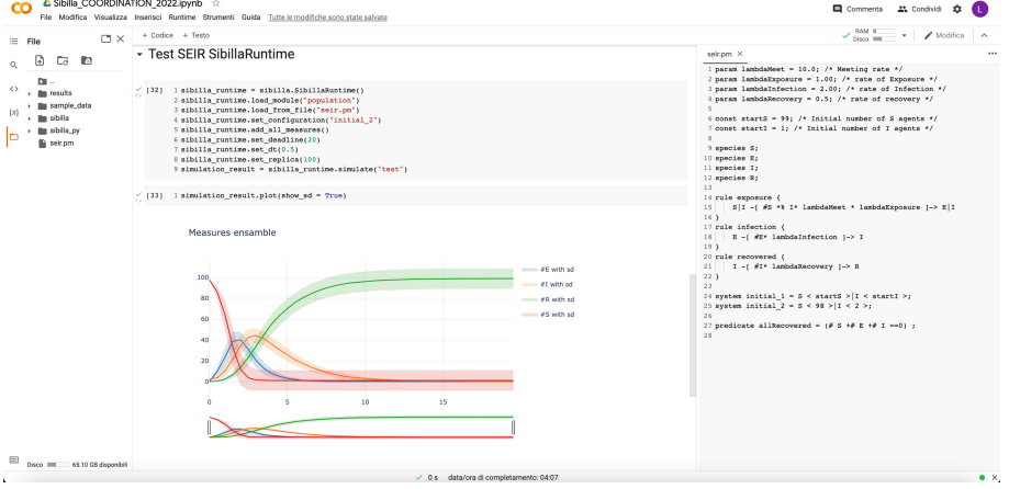
Fig. 1. Sibilla running at Google colaboratory
