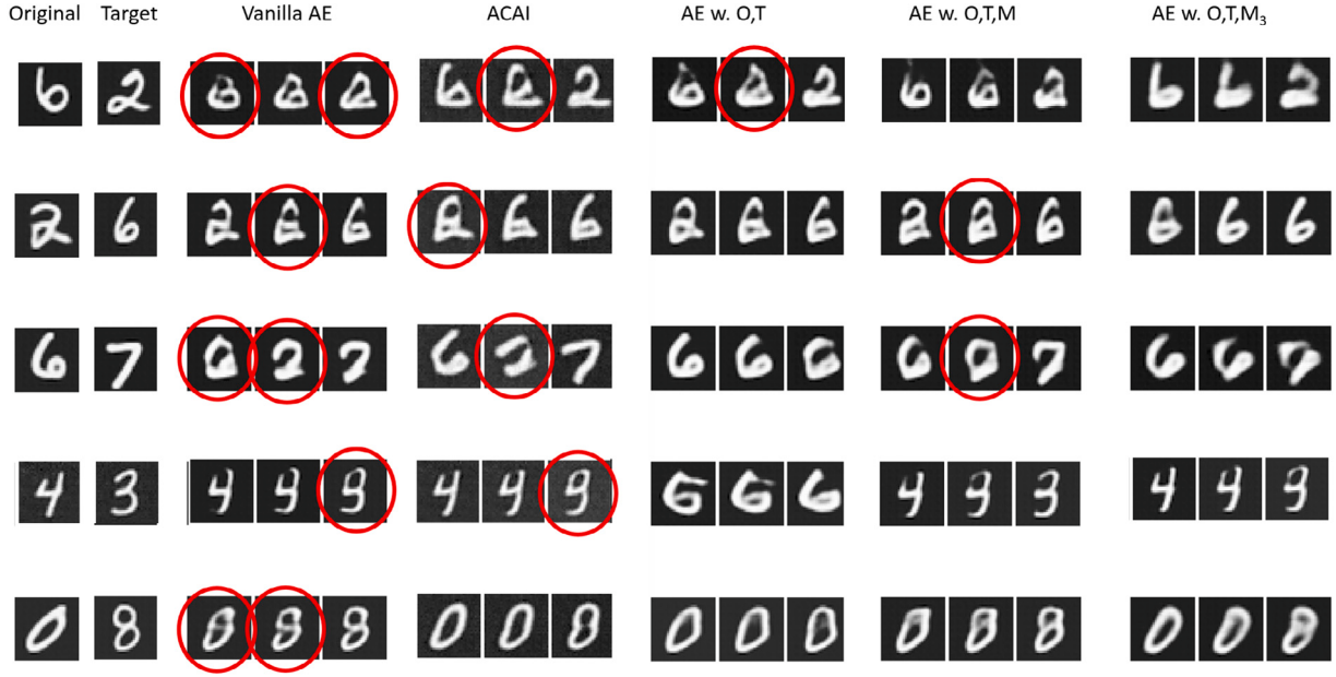
Fig. 4. AS for MNIST for fixed interpolation coefficients b \in \{0.35, 0.5, 0.65\} . Red encircled digits highlight difficult to recognize digits and digits appearing from a class different from the original and target.
