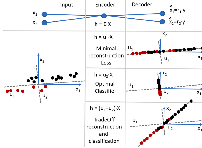
Fig. 2. An AE with optimal encoder h = u_1 \cdot x (and decoder) has lowest reconstruction loss, but it might be impossible or hard for a classifier to classify (autoencoded) samples optimally. Adding a classifier loss of an optimal classifier, e.g., h = u_2 \cdot x , allows trading reconstruction loss for better classification of autoencoded samples.
