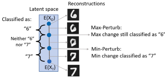
Fig. 3. Illustration of interpolation outcomes and method Max/Min-Perturb. In between two samples X_O, X_T , a reconstructed sample looks very different, potentially being of a class different from Y_O, Y_T .
