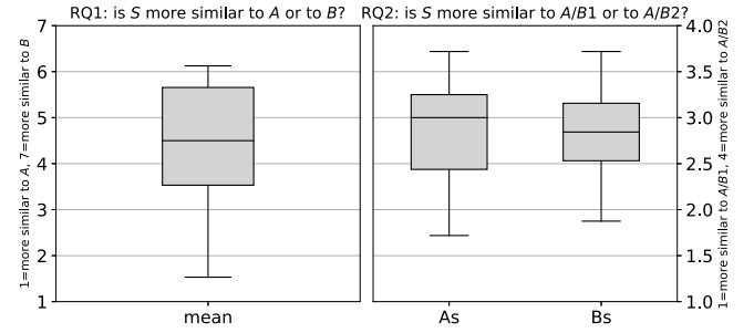
Fig. 7. Results of our user-study. The left plot reflects RQ1, whereas the right plot reflects RQ2. Participants could identify original and target samples significantly better than chance. They were also successfully misled by the AS generated by Max-perturb.
