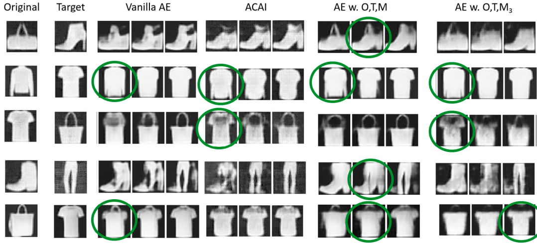
Fig. 5. AS for fashion for fixed interpolation coefficient b \in \{0.35, 0.5, 0.65\} . Green encircled samples have aspects of both the original and target and are well-recognizable.
