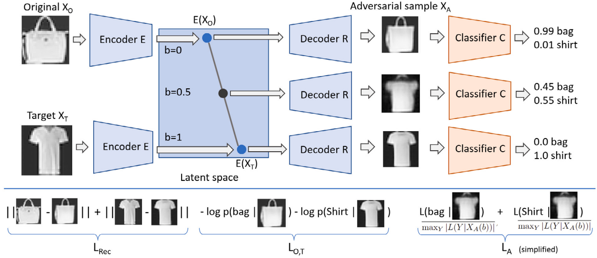
Fig. 1. Outline of our approach. We employ a classifier loss for samples X_A(0) = X_O , X_A(1) = X_T and, possibly, X_A(b) for some b , e.g. b = 0.5 . The classifier helps to regularize the AE.
