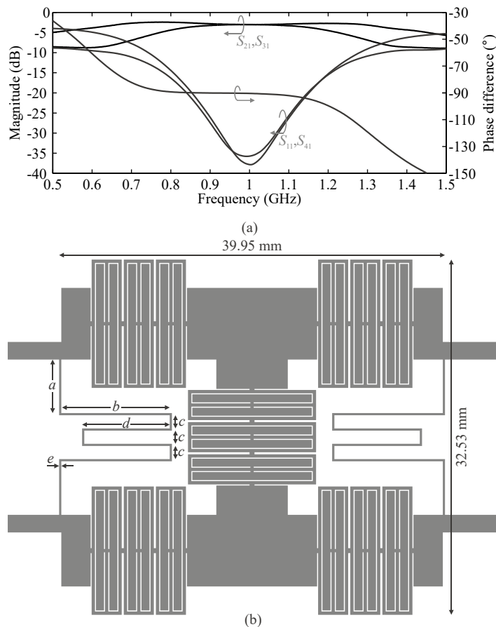
Figure 4: (a) EM-validated frequency performance of the final compact coupler (magnitude of S-parameters of the left axis and phase difference between the coupled and direct ports on the right axis); (b) Layout of the smallest compact coupler: a = 4.15 , b = 8.41 , c = 1.02 , d = 6.64 , e = 0.21 (all dimensions in millimeters).
