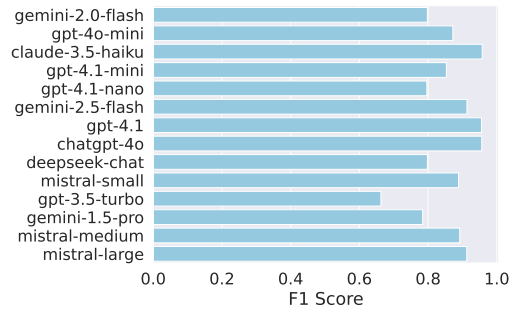
(c) Experiment-3 (LLMs). English only emails.
