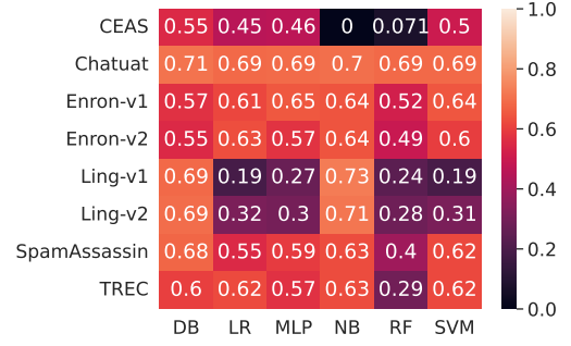
(a) Experiment-1 (cross-Evaluation) English-only emails.
