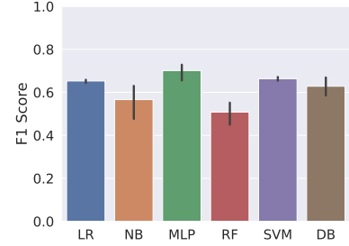
(b) Experiment-2 (all-vs-one). English-only.
