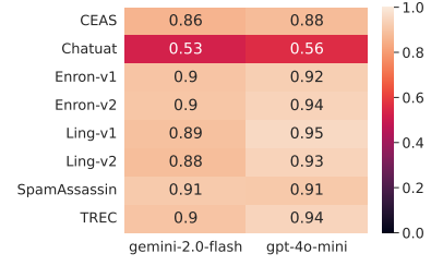
Figure 2: LLM performance (Experiment-3).
