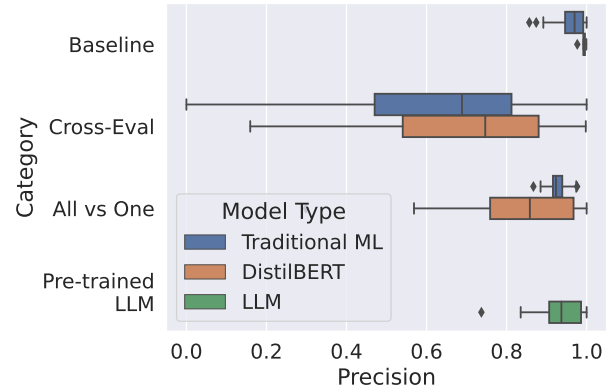
Figure 7: Precision results of our reassessment experiments. Each boxplot represents the distribution of the precision ( \frac{TP}{TP+FP} ) across all of our experiments on existing datasets. For instance, the blue bins show the aggregated results of all the models using feature-based techniques.
