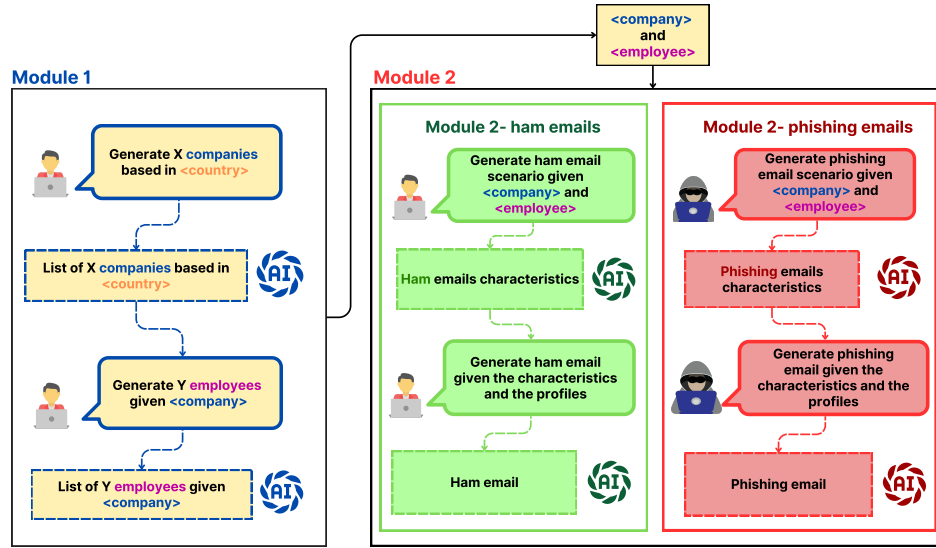
Figure 3: Overview of E-PhishGEN. The framework is composed of two modules: Module 1 generates synthetic company and employee profiles based on high-level input prompts; Module 2 takes these profiles as input and uses an LLM to generate realistic emails, including both benign and phishing variants, tailored to the organizational context and user roles.
