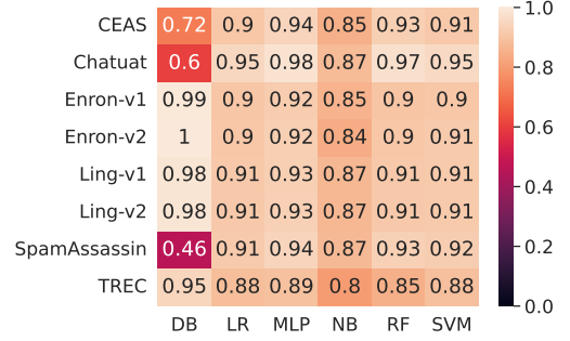
Figure 1: All-vs-one results (Experiment-2). We train each model (columns) on seven datasets, and test it on the left-out dataset (rows).
