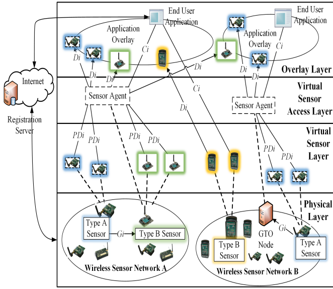
Fig. 1. WSN virtualization architecture
