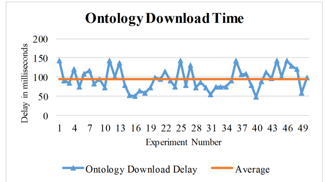
Fig. 9. Ontology Download Time
