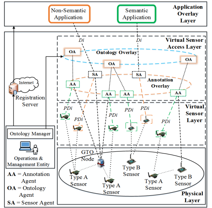
Fig. 2. Proposed data annotation architecture
