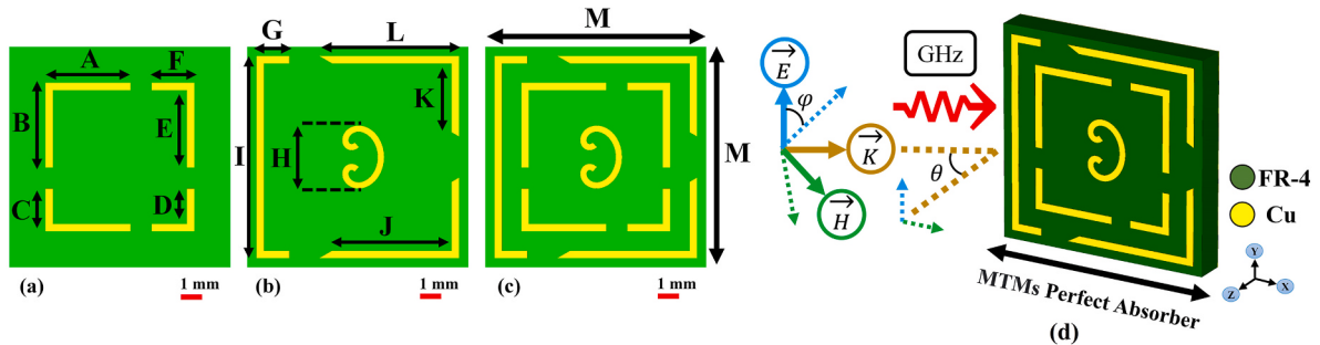
Fig. 1. Conceptual illustration of the proposed metamaterial absorber depicted across three developmental phases: (a) the preliminary structural layout (Design Variant 1), (b) the refined intermediate configuration (Design Variant 2), (c) the fully optimized biosensing geometry (Design Variant 3), (d) schematic illustration of the GHz excitation and multilayer metamaterial absorber biosensor configuration.
