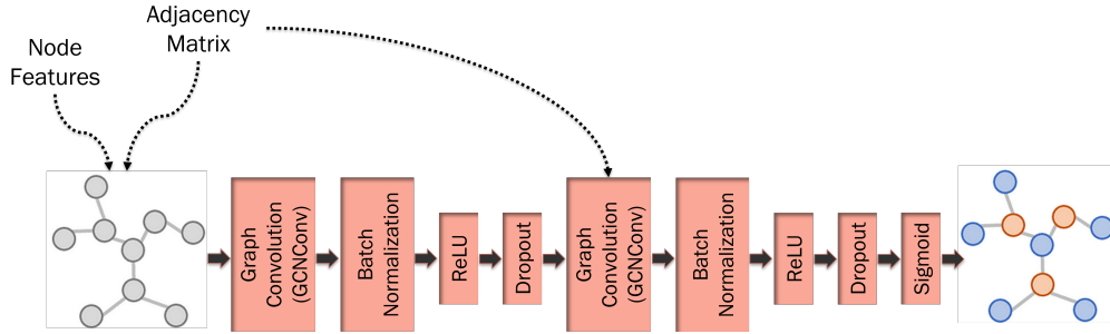
Figure 3.10: Model Architecture
