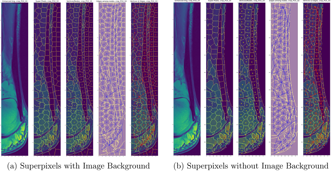
Figure 3.11: Generated Superpixels
