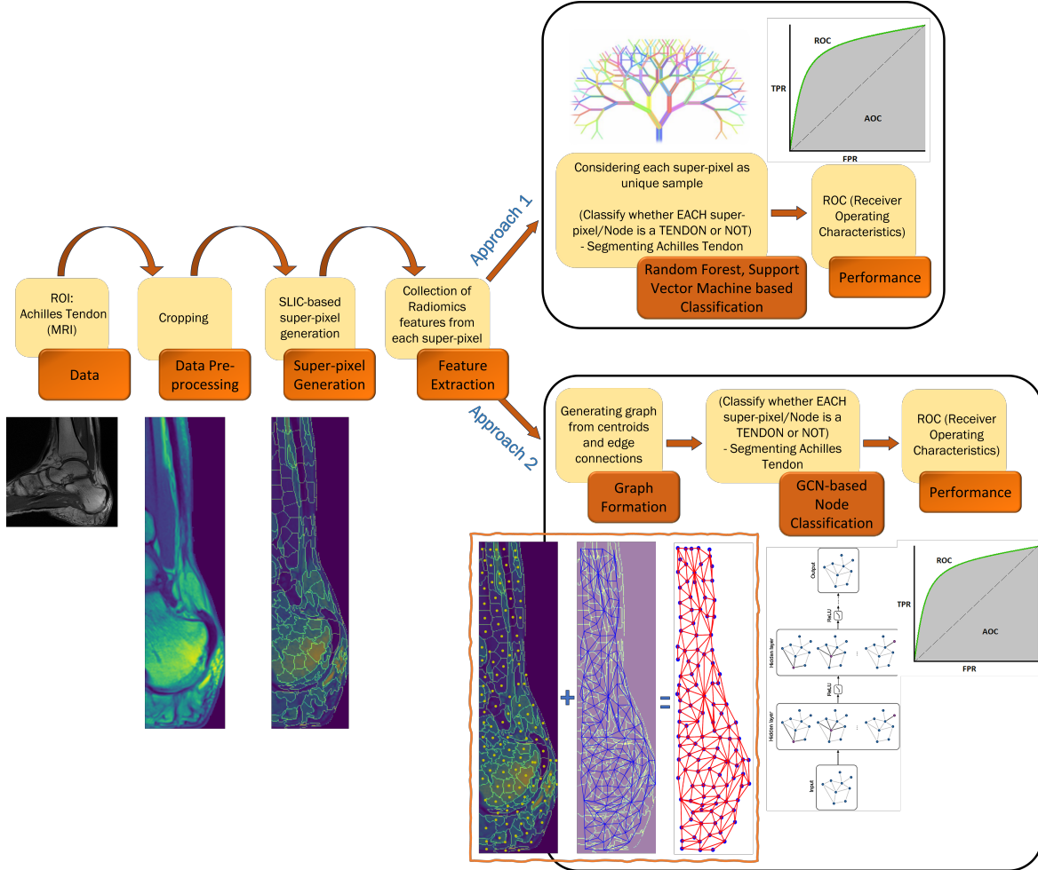
Figure 3.1: Graphical Pipeline
