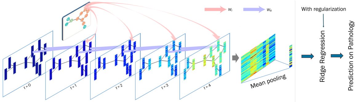
Figure 4.3: Model Architecture [322]
