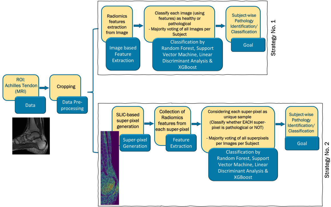
Figure 4.1: Baseline Module
