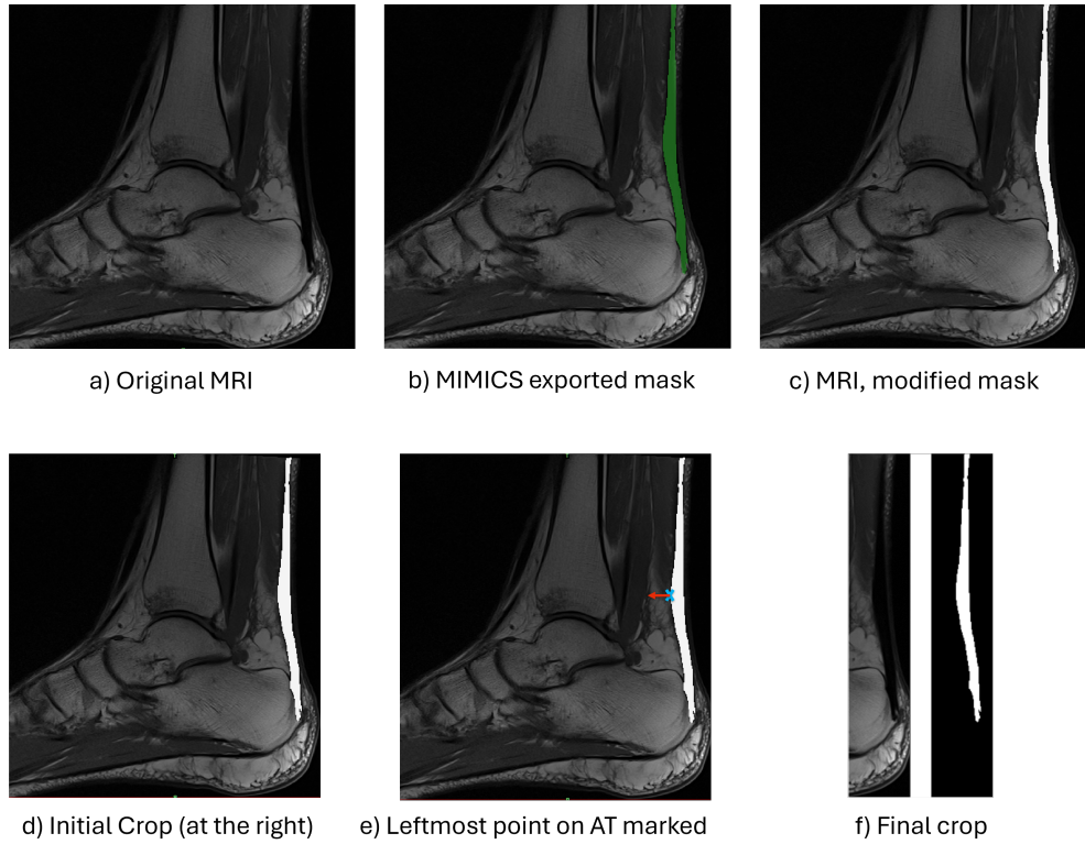
Figure 3.5: Cropping Pipeline
