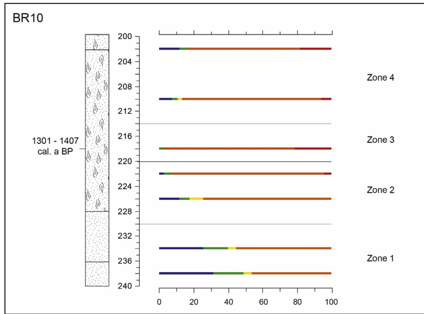
Fig. 9. Summary diatom assemblages and stratigraphic profile for Breiðavík 10 in Breiðavík-Látrar, showing the key environmental changes recorded. For the key, refer to Fig. 4.
