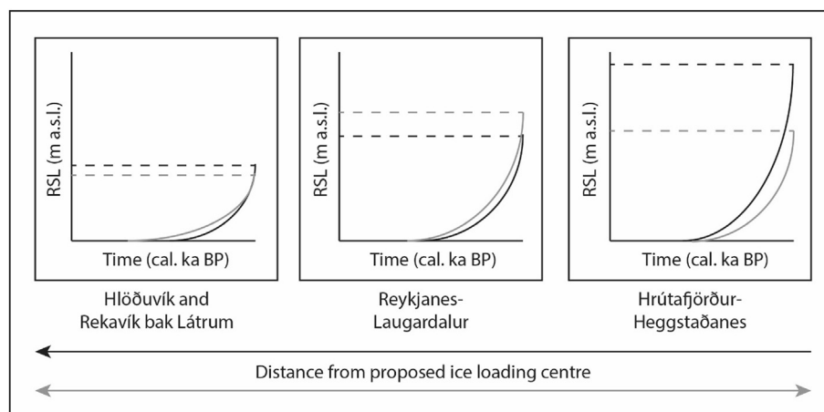
Fig. 3. Hypothesised patterns of RSL change if the centre of uplift was situated in central Iceland or if there was a local centre of uplift in central Vestfirðir in each of the principal research locations – Hlöðuvík and Rekavík bak Látrum, Reykjanes-Laugardalur, and Hrótafjörður-Heggstaðanes – in northwestern Iceland. Under the central Iceland scenario (black), distance from the loading centre increases leftward, whereas distance from the loading centre increases away from Reykjanes-Laugardalur under the local scenario (grey dash). The hypothesized marine limit is denoted by the dashed lines.
