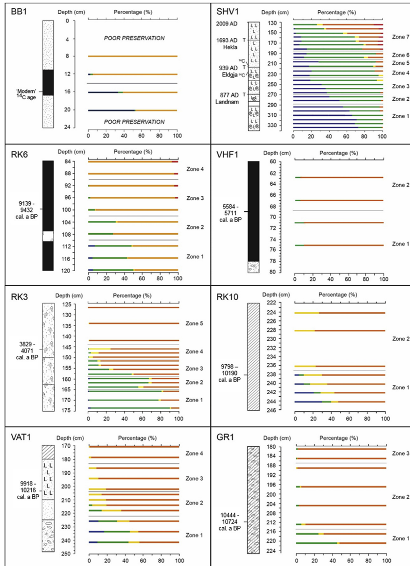
Fig. 7. Summary diatom assemblages and stratigraphic profiles for sites in Reykjanes-Laugardalur showing the key environmental changes recorded in each location: BB1 – Bólvík, SHV1 – Sveinhúsavatn, RK6 – Reykjanes 6, VHF1 – Vatnsfjörður Home Field, RK3 – Reykjanes 3, RK10 – Reykjanes 10, VAT1 – Vatnsfjarðarháls 1, GR1 – Grímhólsvatn. For the key, refer to Fig. 4.
