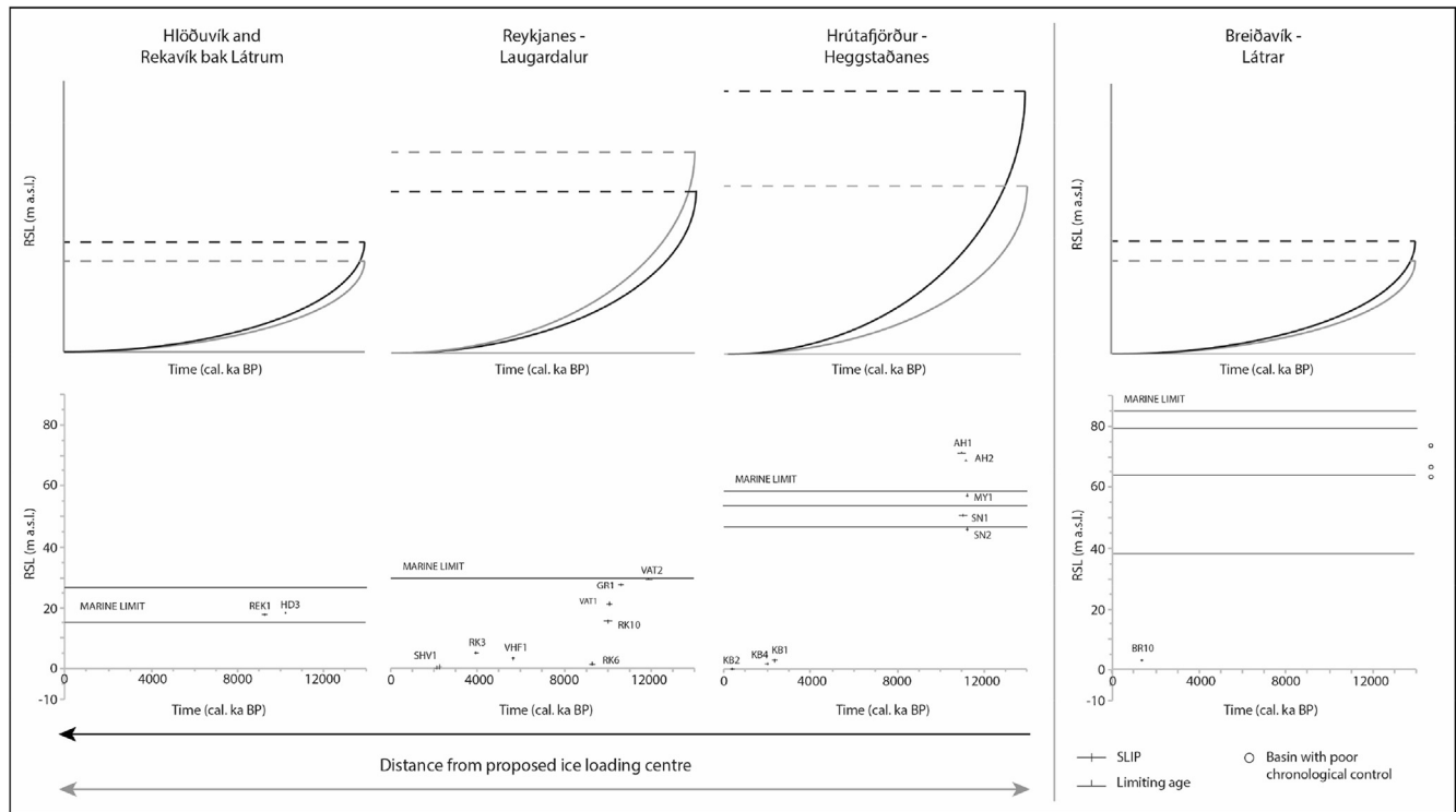
Fig. 6. Hypothesised and reconstructed RSL curves for NW Iceland, based on new and existing data from the region. Hypothesised RSL curves are based on Fig. 3, with grey representing localised uplift and black representing the central uplift scenario. The hypothesised RSL curve for Breiðavík-Látrar is based on its position at an extreme terrestrial location from the principal uplift centre in central Iceland. Reconstructed RSL curves are plotted along the principal research transect in NW Iceland - Hlíðuvík and Rekavík bak Látrum (NW), Reykjanes-Laugardalur (central) and Hrótafjörður-Heggstaðanes (SE) - with Breiðavík-Látrar (SW) plotted separately.
