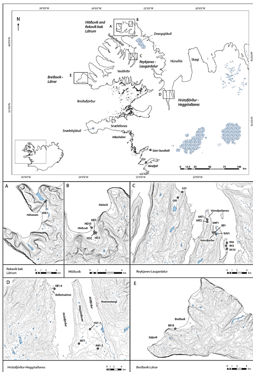
Fig. 2. Study area in NW Iceland, highlighting the key research locations – A: Rekavík bak Látrum, B- Hlíðuvík, C - Reykjanes-Laugardalur, D – Hrutafjörður-Heggstaðanes, E – Breiðavík-Látrar - and sites mentioned in the text. Blue hashed areas – current glaciers, light blue – lakes. Base Map – Based on data from National Land Survey of Iceland. (For interpretation of the references to colour in this figure legend, the reader is referred to the web version of this article.)
