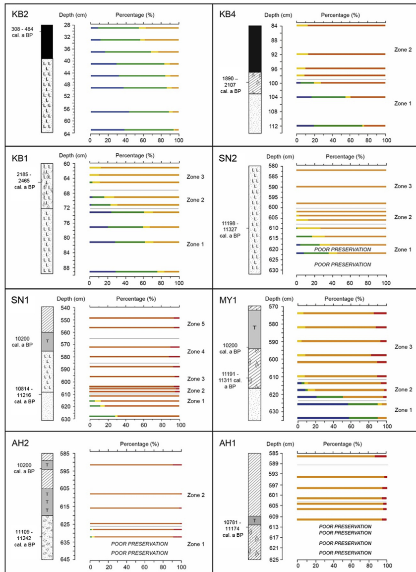
Fig. 8. Summary diatom assemblages and stratigraphic profiles for sites in Hrutafjörður-Heggstaðanes showing the key environmental changes recorded in each location: KB2 – Kolbeinsárnes 2, KB4 – Kolbeinsárnes 4, KB1 – Kolbeinsárnes 1, SN2 – Sandavatn 2, SN1 – Sandavatn 1, MY1 – Mýrar 1, AH2 – Álfhóll 2, AH1 – Álfhóll 1. For the key, refer to Fig. 4.
