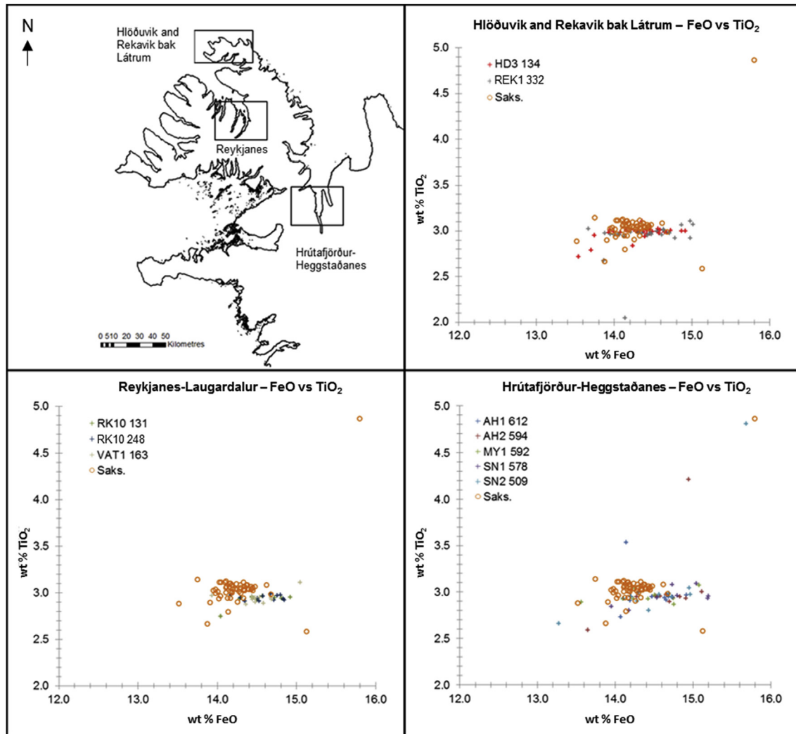
Fig. 5. Geochemical results of tephra analyses on samples from Hlöðuvík and Rekavík bak Látrum, Reykjanes-Laugardalur and Hrótafjörður-Heggstaðanes. Samples are plotted against Saksunarvatn geochemistries (orange circles) sourced from TephraBase (2015) . (For interpretation of the references to colour in this figure legend, the reader is referred to the web version of this article.)
