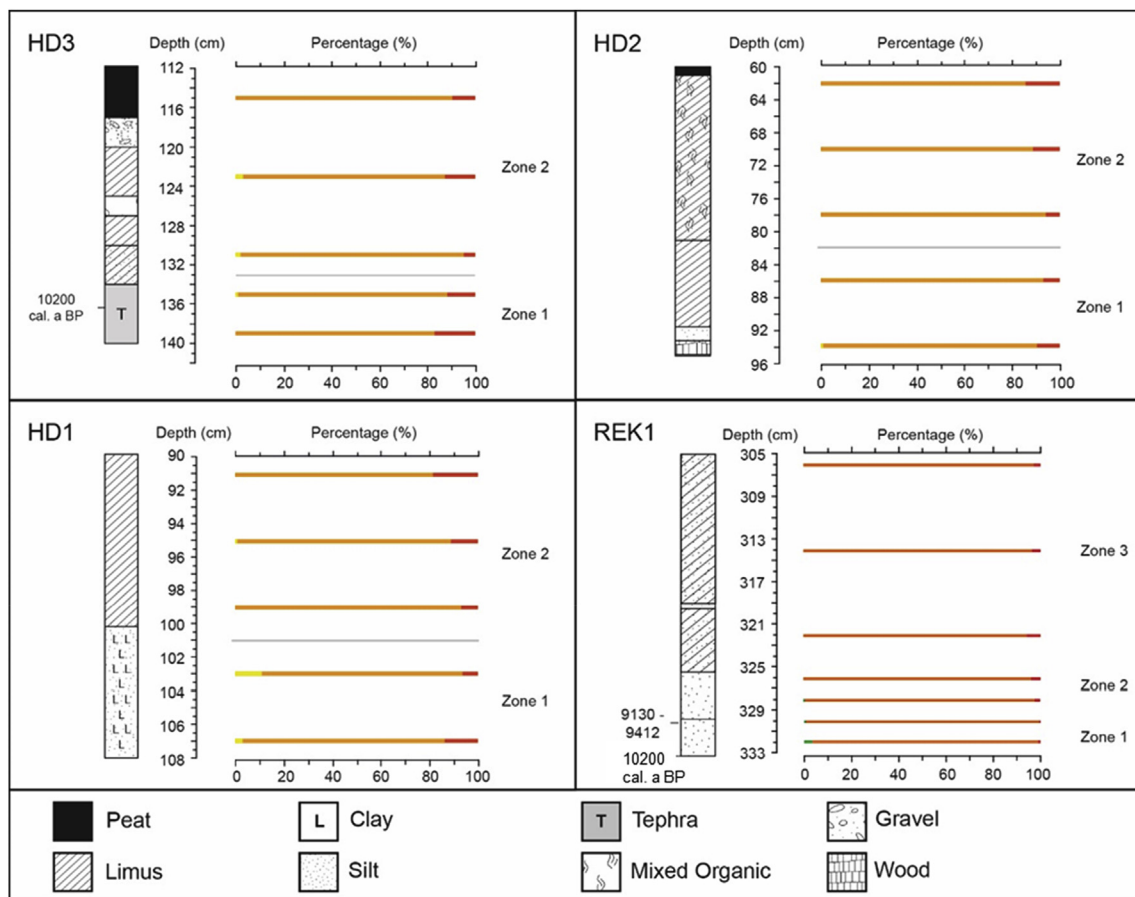
Fig. 4. Summary diatom assemblages and stratigraphic profiles for sites in Hlöðuvík and Rekavík bak Látrum showing the key environmental changes recorded in each location: HD3 – Hlöðuvík 3, HD2 – Hlöðuvík 2, HD1 – Hlöðuvík 1 and REK1 – Rekavík bak Látrum 1. Diatoms are grouped by salinity: blue – marine, green – brackish, yellow – salt tolerant, orange – freshwater, red – salt intolerant. Full diatom assemblages and core stratigraphies are provided in Supplementary Information . (For interpretation of the references to colour in this figure legend, the reader is referred to the web version of this article.)
