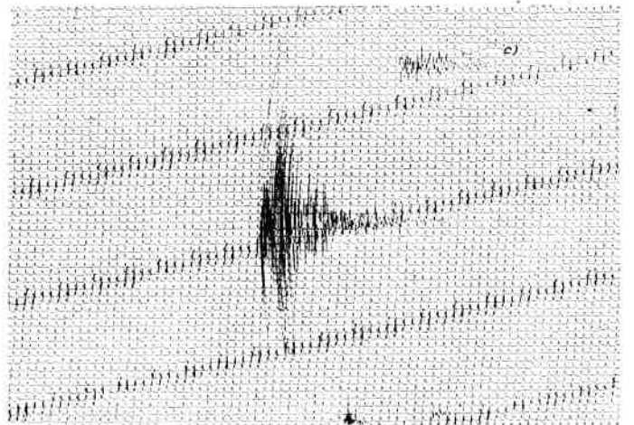
Fig. 2 - Seismogram sections from the stations RI (a) and SN (b and c). The small tick marks are second marks. Typical earthquakes with clear S-waves (a and c) and without S-waves (a and b) can be seen.
