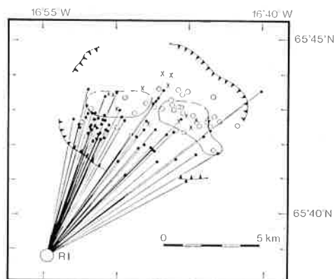
FIG. 3 - S-wave paths to the station RI. Epicenters of earthquakes that are recorded with a clear S-wave are marked with a black dot, open circles denote earthquakes with no recorded S-wave at RI. Earthquakes of intermediate character are marked with X. Areas of maximum attenuation of S-waves are delineated. The caldera fault is drawn after Björsson et al. (1977).
