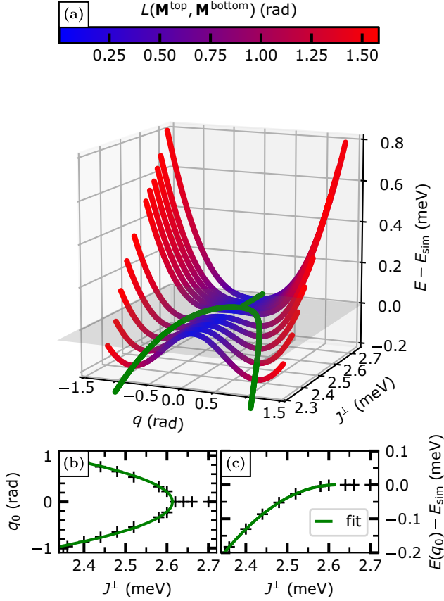
FIG. 11. (a) Local energy landscape along the layer-aligning mode for different J^\perp around the saddle point configurations of bilayer skyrmions in the \alpha\alpha -system. An example for a corresponding eigenvector is shown in Fig. 10(f). The energy is displayed relative to the energy of the simultaneous saddle point configuration E_{\text{sim}} and visualized over the displacement q along the mode. The color code represents the geodesic distance between the magnetizations of the top layer \vec{M}^{\text{top}} and the the bottom layer \vec{M}^{\text{bottom}} . (b,c) Position and value of the local energy minima from (a) recorded over J^\perp . The green lines indicate fits of Eq. (10) and Eq. (11), respectively.
