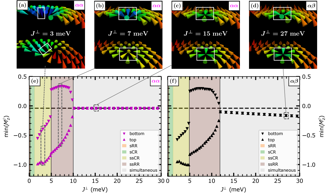
FIG. 17. (a-c) Representation of the saddle point configuration of the bilayer skyrmion collapse in the \alpha\alpha system for J^\perp = 3 meV, J^\perp = 7 meV and J^\perp = 15 meV. The m_z -component of the magnetic moments i is emphasized by the color code. In each layer the magnetic moments i with the minimum m_z -component are highlighted with a white box. (d) Analog representation for the saddle point configuration of a collapse in the \alpha\beta -system for J^\perp = 27 meV. (e) Visualization of the minimum component of the magnetization in the z-direction for collapses of bilayer skyrmions in the \alpha\alpha -system for various J^\perp for both layers l = 1, 2 . The background color indicates the regime of the collapse types as introduced in Sec. IV B. (f) Analog visualization to (e) for the \alpha\beta -system. For comparison the corresponding value for the monolayer skyrmion collapse in Pd/Fe/Ir(111) is indicated as dashed black line in (e) and (f). All calculations were done with the NRE parameter set and only each third data point is shown for better visibility in (e),(f).
