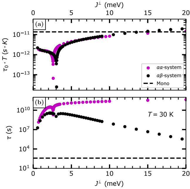
FIG. 15. (a) Temperature independent pre-exponential factor \tau_0 \cdot T (Eq. (6)) for skyrmions in magnetic bilayer systems based on the magnetic monolayer system Pd/Fe/Ir(111) in \alpha\alpha - and \alpha\beta -stacking for various interlayer exchange couplings J^\perp . The dashed line indicates pre-exponential factor for skyrmions within the magnetic monolayer system Pd/Fe/Ir(111) 37 for B = 4.0 T. (b) Skyrmion lifetime \tau for T = 30 K calculated with the Arrhenius law (Eq. (1)) using the energy barriers \Delta E from Fig. 10 (a) and the prefactor \tau_0 displayed in part (a) of this figure.
