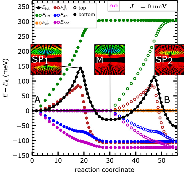
FIG. 5. Minimum energy path for a bilayer skyrmion in the \alpha\alpha -system without interlayer exchange coupling ( J^\perp = 0.0 meV). The total energy is plotted in black. The energy contributions of the different interactions are represented by the color code (see legend). Open circles represent the top Fe layer while filled circles symbolize the bottom Fe layer. The spin configuration of the saddle points (SP 1 and SP 2 ) is shown as well as the spin configuration of the intermediate minimum (M). For the configuration of the initial bilayer skyrmion A and the final field polarized state B see the Insets in Fig. 2.
