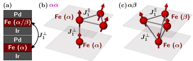
FIG. 1. (a) Magnetic bilayer systems built from two units of the system Pd/Fe/Ir(111). Two different stackings ( \alpha\alpha and \alpha\beta ) are considered which correspond to atoms of the two hexagonal Fe layers being on top of each other or shifted with respect to each other. (b,c) Schematic representation of the nearest-neighbor intralayer ( J_1^\parallel ) and interlayer ( J_1^\perp ) exchange bounds for the \alpha\alpha -stacked and \alpha\beta -stacked magnetic bilayer, respectively. The bonds are indicated through the connections of the red magnetic moments.
