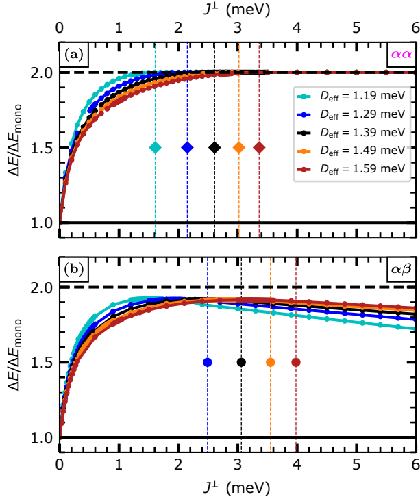
FIG. 18. (a,b) Energy barrier \Delta E of bilayer skyrmions in the \alpha\alpha - and \alpha\beta -system for various interlayer exchange couplings J^\perp relative to the energy barrier of a skyrmion in the underlying monolayer system \Delta E_{\text{mono}} . The variation of the DMI is indicated through the color code in the legend. (a) displays the \alpha\alpha - and (b) presents the \alpha\beta -system. The vertical dashed lines indicate the positions of J_C^\perp (See Fig. 10). These critical interlayer exchange couplings J_C^\perp are displayed in dependence of \Delta E_{\text{mono}} in Fig. 13.
