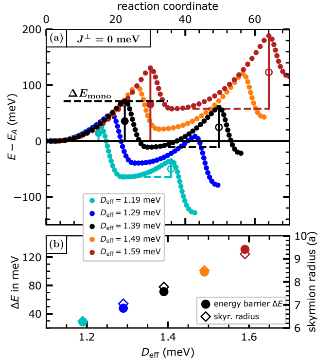
FIG. 12. (a) Minimum energy paths of bilayer skyrmions in the \alpha\alpha -system based on the effective parameters from the monolayer system Pd/Fe/Ir(111) for different values of the DMI (see color code in legend). The interlayer exchange constant is set to zero ( J^\perp = 0.0 meV). For comparison the energy barrier of the skyrmion in the magnetic monolayer for D_{\text{eff}} = 1.39 meV 31 is indicated as dashed line. (b) Energy barriers and radius of the bilayer skyrmions in the magnetic monolayer systems for different values of the DMI. The radius of the relaxed bilayer skyrmion is given in units of the lattice constant a .
