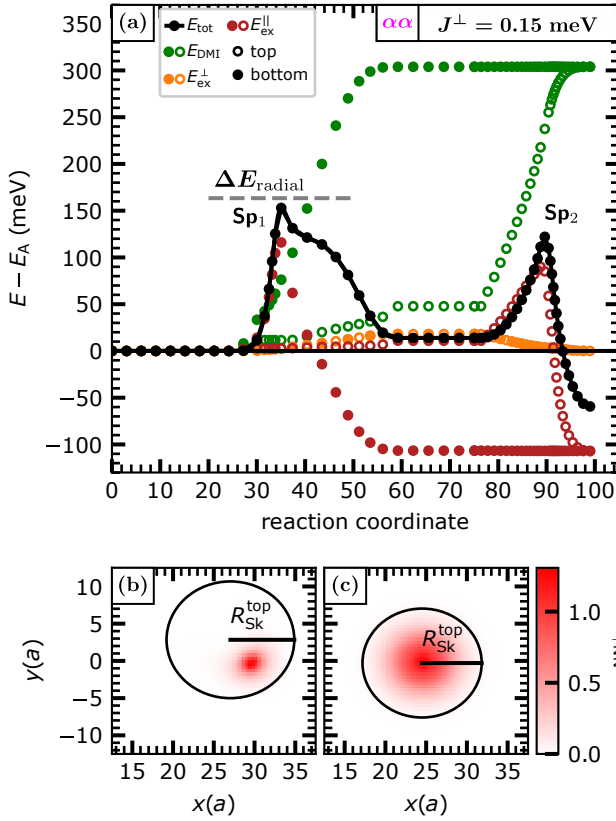
FIG. 6. (a) Minimum energy path for a bilayer skyrmion in the \alpha\alpha system with interlayer exchange coupling ( J^\perp = 0.15 meV). The energy contributions of the different interactions are represented by the color code (see legend). Open circles represent the top Fe layer while filled circles symbolize the bottom Fe layer. The first saddle point corresponds to a chimera collapse (cf. Fig. 4(e-h)). The energy barrier corresponding to the meta-stable radial saddle point configuration is visualized by the dashed gray line. (b,c) The interlayer exchange energy costs f(\vartheta_i^{\text{NN}_i^\perp}) are presented by the color code versus the in-plane directions, where a is the in-plane lattice constant. The skyrmion radius R_{\text{Sk}}^{\text{top}} and the position of the unchanged layer (top layer in this example) during the first part of the collapse is represented by a circle. While (b) belongs to the chimera collapse saddle point configuration (c) represents the saddle point of the meta-stable sRR collapse for J^\perp = 0.15 meV.
