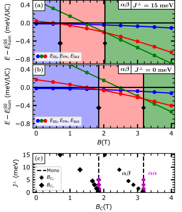
FIG. 3. (a) Zero temperature phase diagram for the \alpha\beta system for J^\perp = 15.0 meV. The critical fields B_{C_1} and B_{C_2} define the phase transitions between the spin spiral phase (SS, blue), the skyrmion lattice phase (SkX, red) and the field polarized phase (FM, green), respectively. The energy is defined per unit cell and displayed relative to the energy of the minimum of the dispersion of homogeneous spin spirals. The background color represents the phases in a certain magnetic field range. (b) Analog visualization of the phase diagram for the \alpha\beta system for J^\perp = 0 meV. (c) Critical magnetic fields B_{C_1} or B_{C_2} for different values of J^\perp for the \alpha\alpha and \alpha\beta system. The reference of the magnetic monolayer system Pd/Fe/Ir(111) is plotted as a dashed line.
