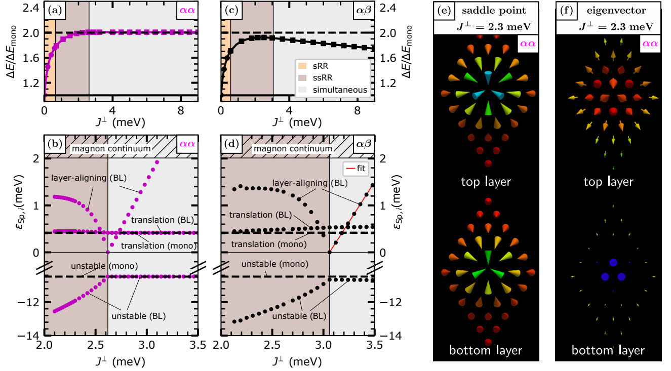
FIG. 10. (a,c) Energy barriers of bilayer skyrmions in the \alpha\alpha and the \alpha\beta system relative to the energy barrier of skyrmions within the magnetic monolayer system Pd/Fe/Ir(111) for various interlayer exchange constants J^\perp . The effective parameter set (cf. Tab. I) is used and the background colors follow the definition of the collapse mechanisms as defined in Fig. 9 for the NRE model. For better visibility every third data point is displayed. (b,d) Visualization for the \alpha\alpha and \alpha\beta system, respectively, of the lowest eigenvalues of the Hessian of the saddle point configuration which belong to the energy barriers displayed in (a,b) for various J^\perp . The identified eigenmodes calculated for the bilayer system are labeled with BL. For a detailed description see the text. The dashed lines indicate the eigenvalues for a skyrmion in the monolayer system at B = 4.0 T described with the effective model 37 . In (d) a fit following Eq. (13) is presented by a red line. (e) Representation of the saddle point configuration for the bilayer skyrmion in the \alpha\alpha system for J^\perp = 2.3 meV. (f) Visualization of the eigenvector for the layer-aligning mode of the saddle point presented in (e). The color code represents the z-component of the orientation of the vectors.
