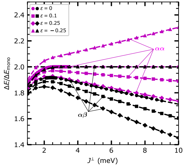
FIG. 16. Energy barriers of bilayer skyrmions in \alpha\alpha - (magenta) and \alpha\beta -systems (black) relative to the energy barrier of the skyrmion in the magnetic monolayer Pd/Fe/Ir(111) depending on the interlayer exchange per unit cell J^\perp . The effective model was used to describe the intralayer exchange coupling. The different values of \epsilon encode different distributions of the interlayer exchange to the first neighbor and second neighbor shell (See Eq. 14 and Eq. 15). A value \epsilon < 0 indicates a frustrated system in terms of interlayer exchange coupling.
