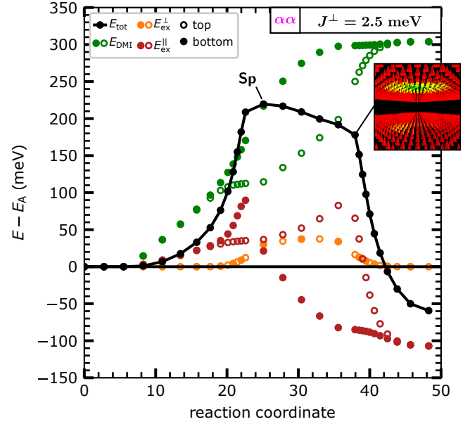
FIG. 7. Minimum energy path for a bilayer skyrmion in the \alpha\alpha -system with interlayer exchange coupling ( J^\perp = 2.5 meV). The energy contributions of the different interactions are represented by the color code (see legend). Open circles represent the top Fe layer while filled circles symbolize the bottom Fe layer. An exemplary spin configuration in the region of the collapse of the second skyrmion is shown as an inset. For the spin configuration of the actual saddle point see Fig. 4(i-l)
