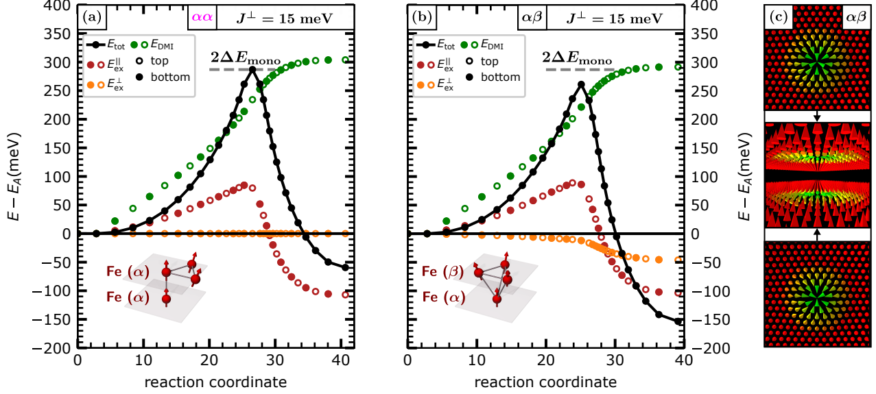
FIG. 8. (a) Minimum energy path for a bilayer skyrmion in the \alpha\alpha -system with interlayer exchange coupling ( J^\perp = 15.0 meV). The energy contributions of the different interactions are represented by the color code (see legend). Open circles represent the top Fe layer while filled circles symbolize the bottom Fe layer. Twice the energy barrier of a skyrmion in the corresponding monolayer system Pd/Fe/Ir(111) is shown as dashed gray line. The inset displays schematically the stacking of the Fe layers. (b) Analog visualization of the minimum energy path for the \alpha\beta -system for J^\perp = 15 meV. (c) The spin configuration of the saddle point for the collapse of the bilayer skyrmion in the \alpha\beta -system is shown. For the corresponding configuration of the \alpha\alpha -system see Fig. 4(m-p).
