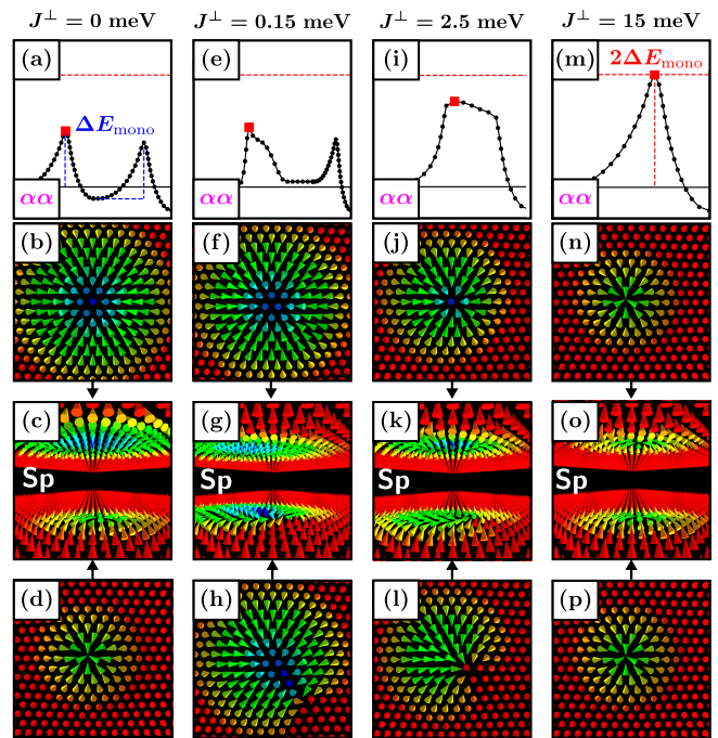
FIG. 4. Representation of collapse mechanisms for bilayer skyrmions in the \alpha\alpha -system for different interlayer exchange couplings J^\perp . The top row shows the total energy along the minimum energy path, while the first occurring saddle point is marked in red. The blue (red) dashed line represents the energy barrier (twice the energy barrier) of a skyrmion in the magnetic monolayer system Pd/Fe/Ir(111) 31 . Below the spin configuration of the corresponding saddle point is visualized. (a-d) Successive radial-radial collapses of the bilayer skyrmion for J^\perp = 0 meV. (e-h) Successive chimera-radial collapse for J^\perp = 0.15 meV. (i-l) Chimera type collapse in one layer with shrunken skyrmion in the other layer for J^\perp = 2.5 meV. This collapse is called semi-successive chimera-radial collapse. (m-p) Simultaneous radial collapse for J^\perp = 15 meV.
