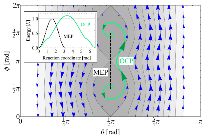
Figure 4. Distribution of the torque (blue arrows) generated by the internal field of the macrospin system with both easy and hard anisotropy axes, superimposed on the contour plot showing the energy surface of the system defined by Eq. (13). The green line shows the calculated OCP for T = 0.32\tau_0 and \alpha = 0 . Green arrows indicate the velocity of the system. The size of the blue (green) arrows code the magnitude of the torque (velocity). Black dashed line shows the minimum energy path (MEP). The inset shows the energy of the system as a function of displacement along the OCP (green solid line) and MEP (black dashed line).
