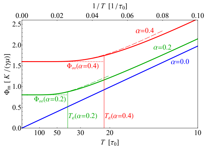
Figure 3. Minimum energy cost of magnetization switching as a function of the inverse of the switching time. Dashed (dotted) lines show long (infinite) switching time asymptotics. Thin vertical lines indicate switching time T_\varepsilon , for which the minimum energy cost is \varepsilon = 10\% larger than the infinite switching time limit \Phi_\infty .
