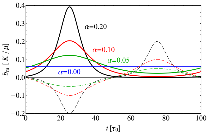
Figure 2. Amplitude of the switching field as a function of time for T = 100\tau_0 and several values of \alpha (solid lines). Dashed lines show \alpha b_i^\perp , which is proportional to the polar component of the torque generated by the internal field.
