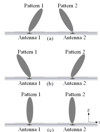
FIGURE 2. Schematic diagram of the antenna beam pattern: (a) correlated antennas, (b) uncorrelated antennas in the presence of mutual coupling, (c) uncorrelated antennas as the elements of an ideal array.
