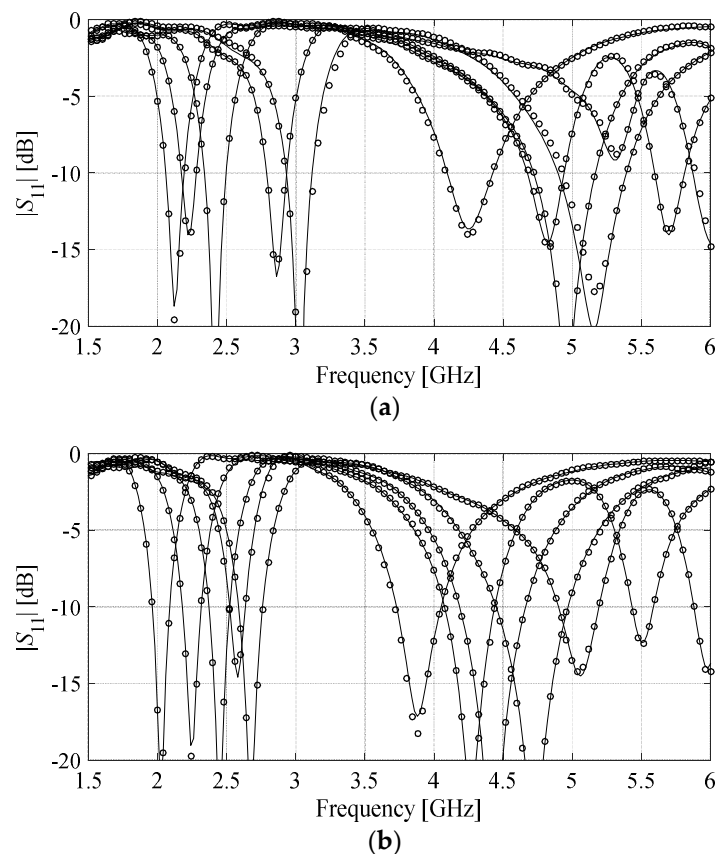
Figure 6. Reflection characteristics of the antenna of Figure 5 at the selected test locations, i.e., full-wave electromagnetic simulation response (—) and the proposed PCA-based surrogate (o). (a) Surrogate model established using two principal components ( X_S = X_2 ) and 50 training data samples; (b) Surrogate established using three principal components ( X_S = X_3 ) and 200 training data samples.
