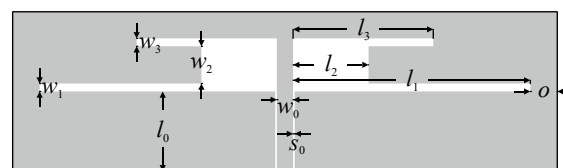
Figure 5. Dual-band dipole antenna: geometry [43].
