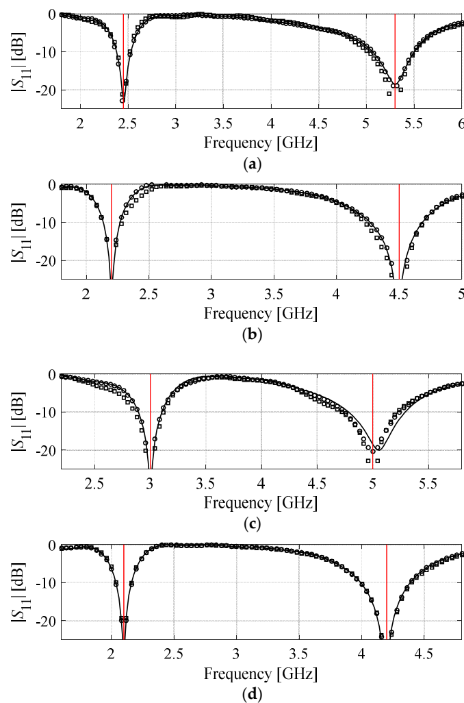
Figure 7. Reflection characteristics of the antenna of Figure 5, i.e., PCA-based surrogate (o), nested kriging surrogate [40] ( \square ), and full-wave simulation at the design rendered through optimization of the PCA-based model (—). The following target vectors were considered: (a) f_1 = 2.45 GHz, f_2 = 5.3 GHz, (b) f_1 = 2.2 GHz, f_2 = 4.5 GHz, (c) f_1 = 3.0 GHz, f_2 = 5.0 GHz, and (d) f_1 = 2.1 GHz, f_2 = 4.2 GHz. Vertical lines denote the target operating frequencies of the antenna.
