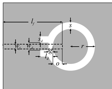
Figure 8. Geometry of the ring slot antenna [43]. The feeding line marked using the dashed line.
