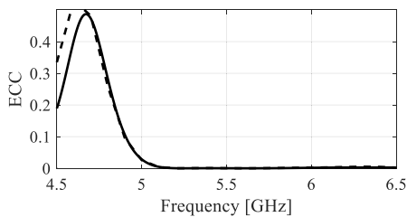
FIGURE 13. Envelop correlation coefficient. Simulated (—), and calculated (---).
