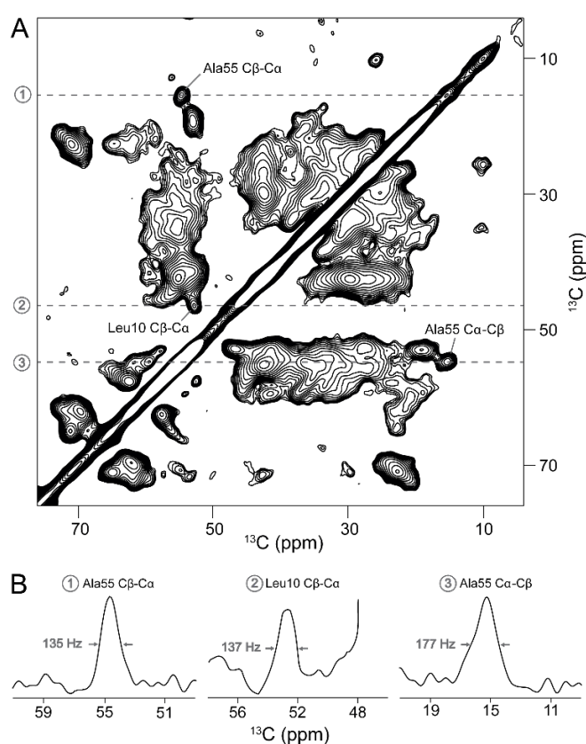
Fig. 3 DNP enhanced ^{13}\text{C} - ^{13}\text{C} correlation spectrum of microcrystalline SH3 at 100 MHz carbon frequency (at 9.4 T), recorded at 181 K. (A) 2D ^{13}\text{C} - ^{13}\text{C} DARR spectrum recorded with 25 ms mixing time. The dashed lines indicate positions of cross sections for evaluation of line widths. (B) Cross sections for selected cross peaks as indicated in (A), along with their line widths. To enable the evaluation of line width, the spectrum was recorded with a sufficiently long acquisition time and processed without application of a window function in F_2 .
