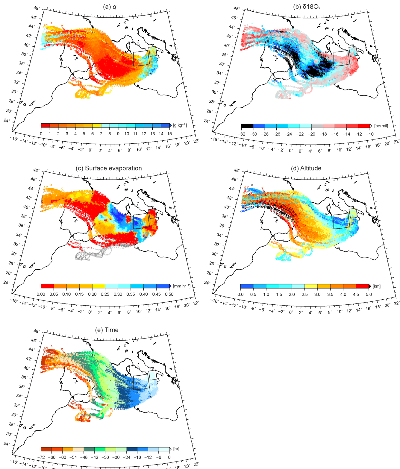
Figure 7. History of air parcel arriving at SI in the 800–700 hPa layer at 20:00 UTC on 15 October 2012. (a) Water vapour mixing ratio, q (g kg -1 ), (b) \delta^{18}\text{O}_v (‰), (c) surface evaporation (mm h -1 ), (d) altitude (km), and (e) time (h).
