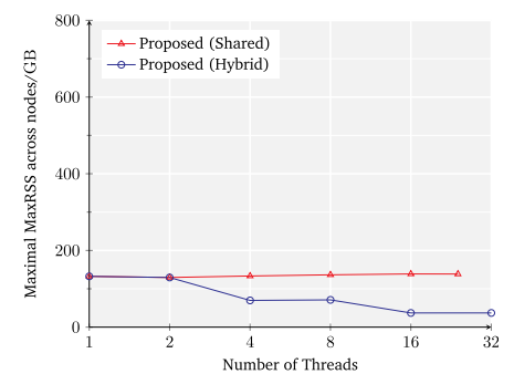
(l) Memory consumption ESO 32bpp
