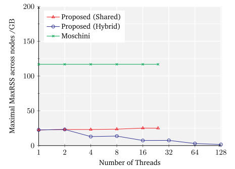
(c) Memory consumption Naples
