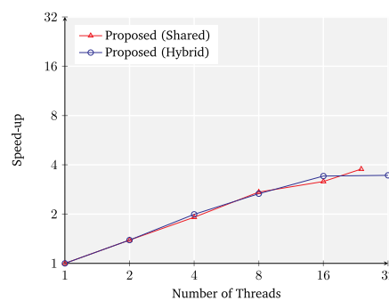
(k) Speed-up ESO 32bpp
