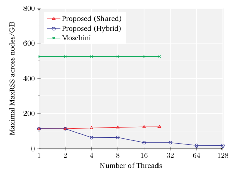
(i) Memory consumption ESO 16bpp
