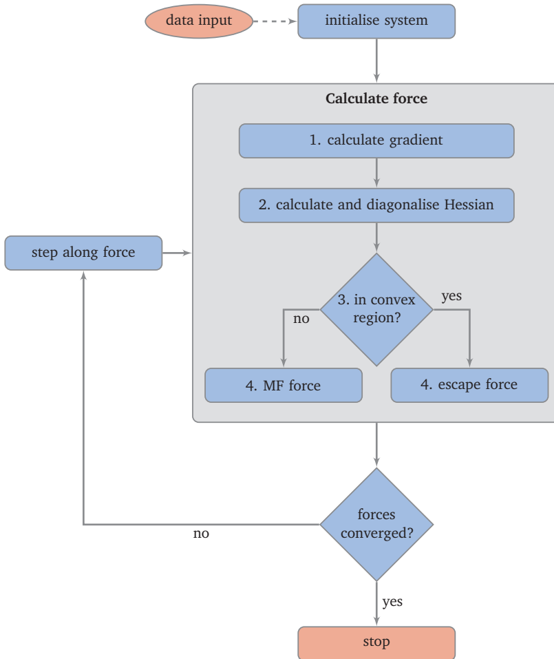
FIGURE 2.2 – Flow chart of the MMF algorithm
