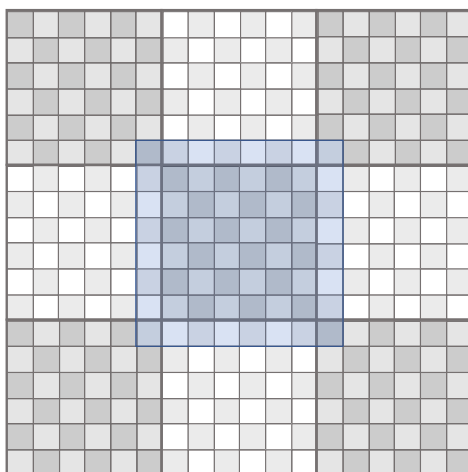
FIGURE 3.8 – Checkerboard domain decomposition for parallelised Monte Carlo
