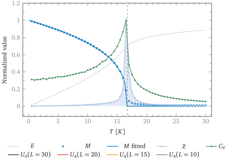
FIGURE I.8 – Monte Carlo test system
