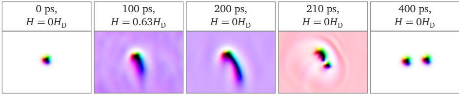
FIGURE 2.11 – Dynamics simulation of skyrmion duplication
