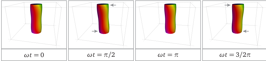
FIGURE 2.3 – Eigenmode of a skyrmion tube
