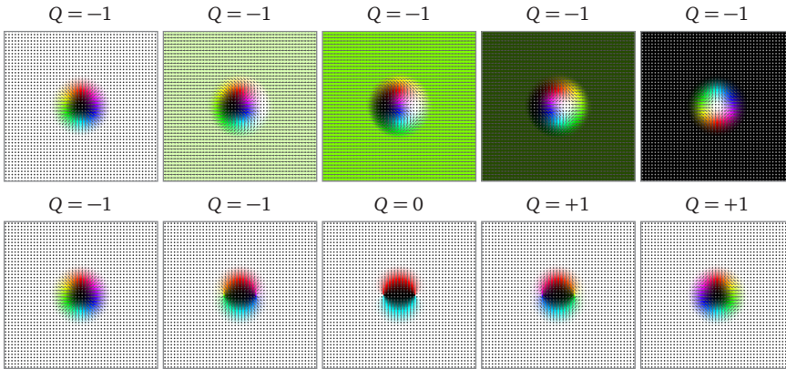
FIGURE 1.11 – Transformations between a skyrmion and an antiskyrmion
