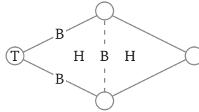
FIGURE 1.28 – Schematic of skyrmion collapse saddle points in the hexagonal unit cell
