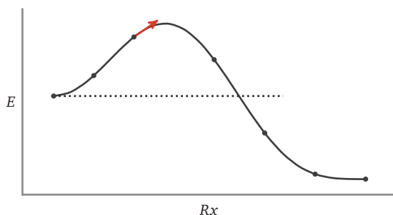
FIGURE 1.5 – Climbing image method
