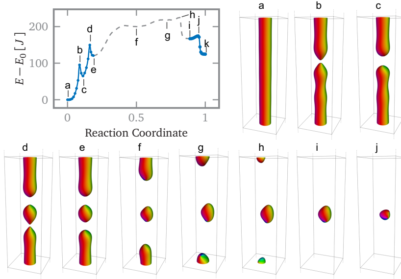
FIGURE 4.10 – Globule collapse GNEB Path
