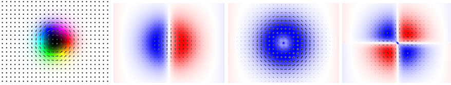
FIGURE 2.7 – Lowest three eigenmodes of an isolated skyrmion
