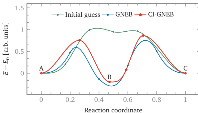
FIGURE 1.8 – Single spin energy barriers
