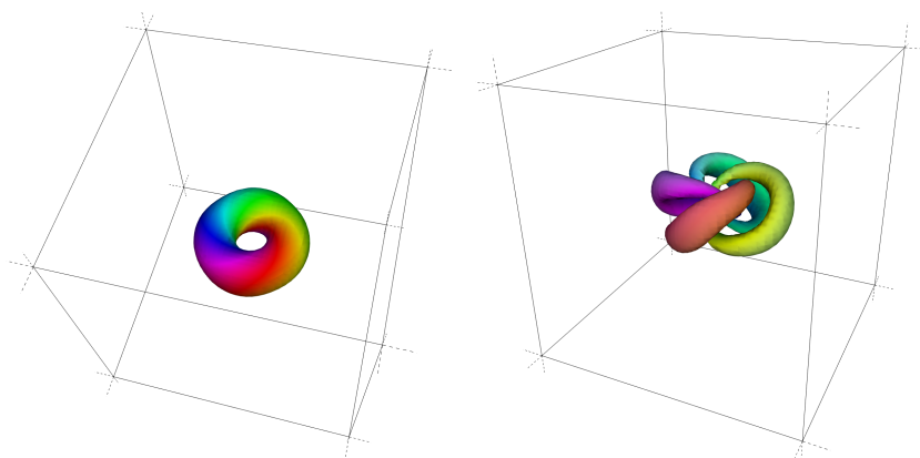
FIGURE 3.17 – Hopfion isosurface visualisations
