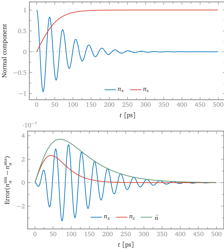
FIGURE 1.12 – LLG dynamics: damped spin precession
