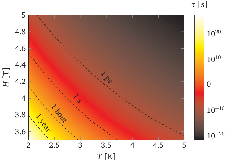
FIGURE 1.29 – HTST Arrhenius plot for the skyrmion collapse
