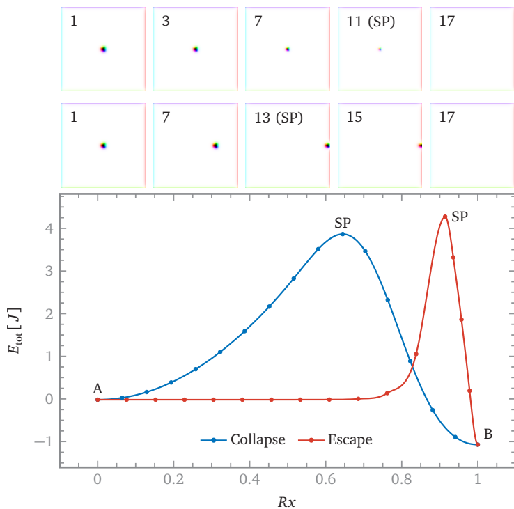
FIGURE 1.9 – Skyrmion transitions: minimum energy paths
