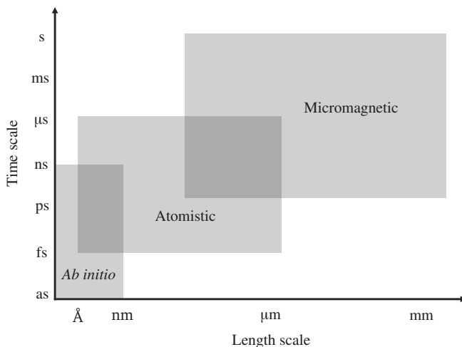
FIGURE I.5 – Hierarchy of time and length scales
