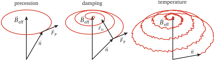
FIGURE I.10 – Schematic of spin movement under LLG equation
