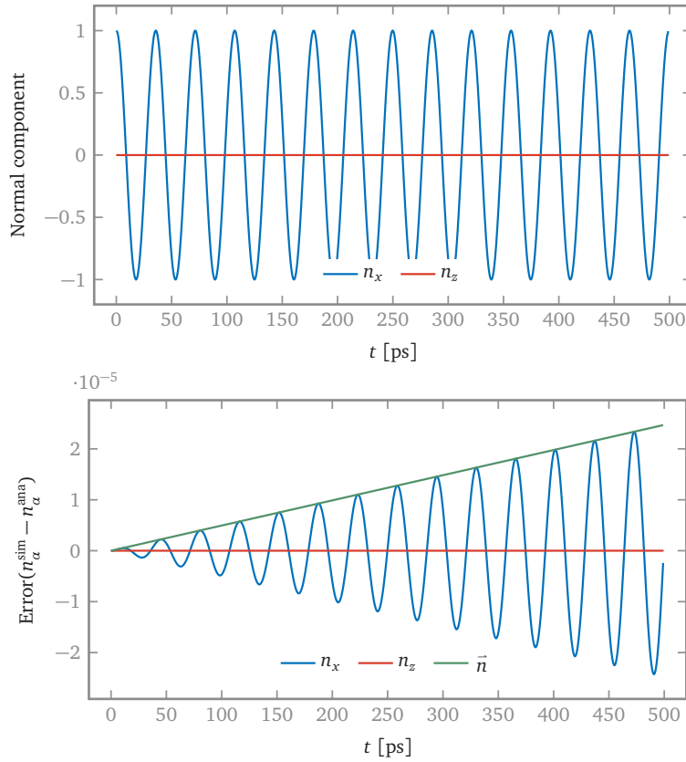
FIGURE I.11 – LLG dynamics: spin precession without damping
