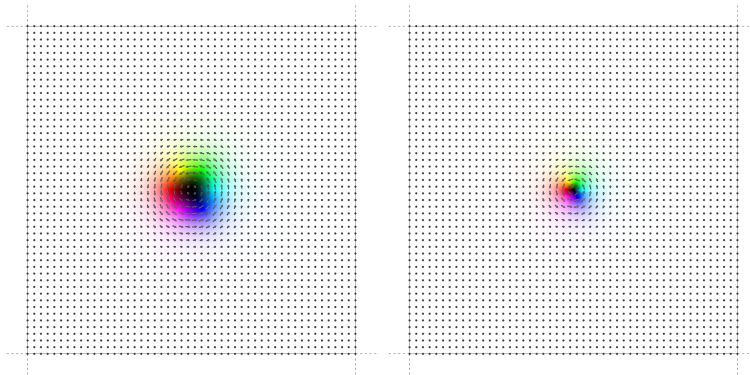
FIGURE 1.26 – Skyrmion and collapse saddle point in simple cubic lattice Simple cubic lattice with periodical boundary conditions, containing a single Bloch skyrmion (left) and the saddle point configuration for the radial skyrmion collapse (right).
