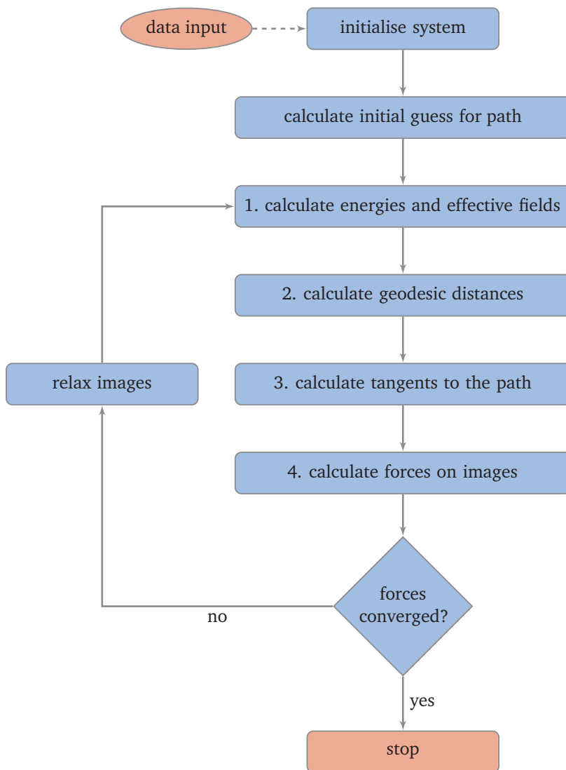
FIGURE 1.3 – Flow chart of the GNEB algorithm
