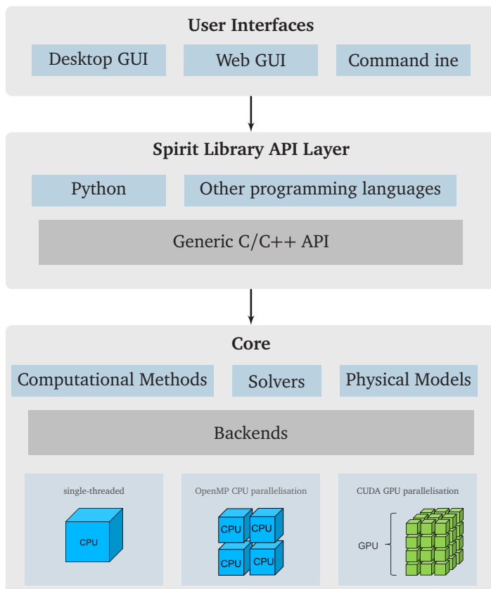
FIGURE 3.1 – Schematic of Spirit code structure
