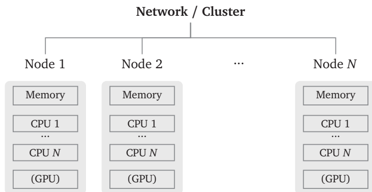
FIGURE 3.7 – Schematic of parallelisation over multiple nodes
