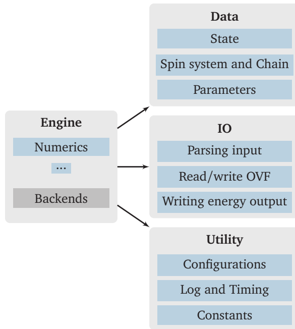
FIGURE 3.4 – Schematic of Spirit core library layout
