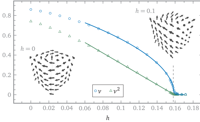
FIGURE 3.9 – Stray field-caused vorticity of a cube
