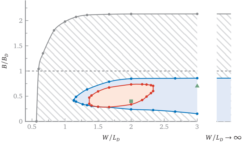
FIGURE 4.9 – Stability of the globule in an infinite nanowire
