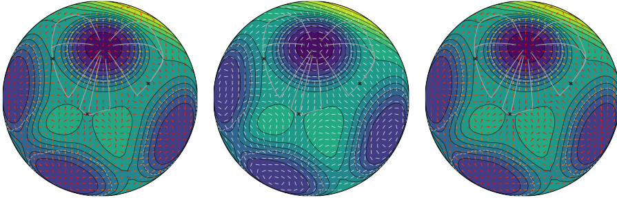
FIGURE 2.5 – Spherical plot of the mode following force contributions
