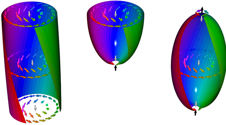
FIGURE 4.4 – Comparison of skyrmion bobber and globule
