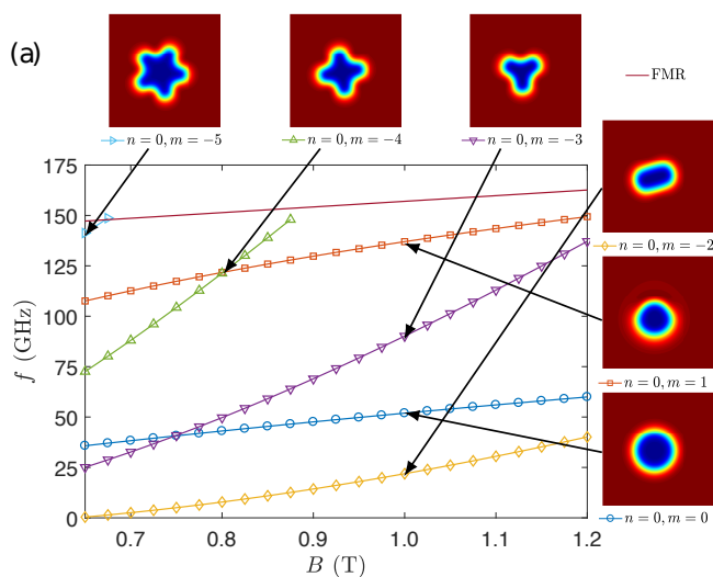
FIGURE 1.25 – Dynamical skyrmion modes
