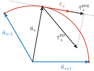
FIGURE 1.4 – Path tangents projection
