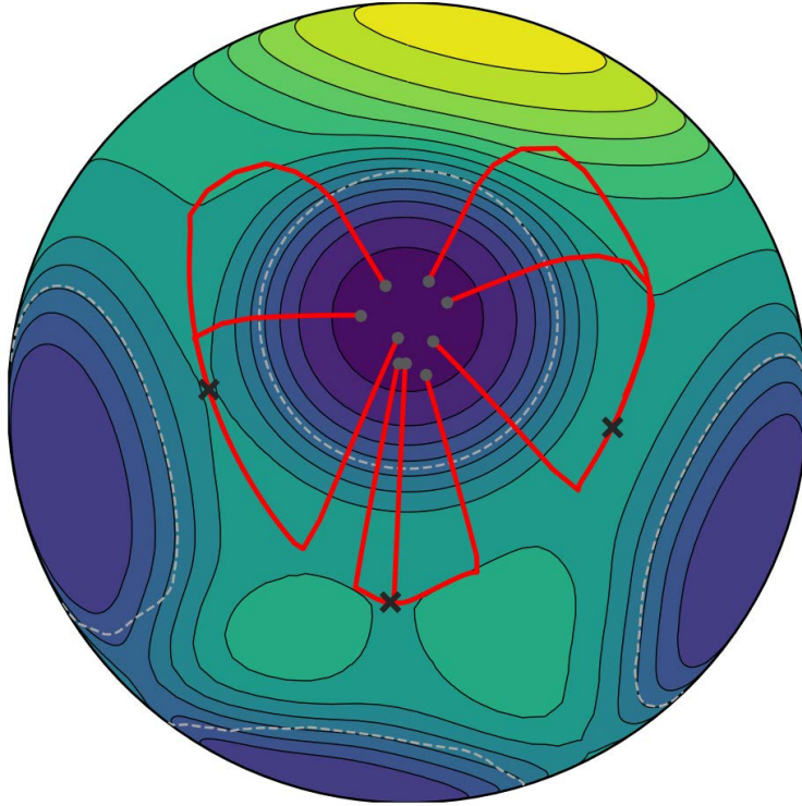
FIGURE 2.4 – Mode following path of a single spin
