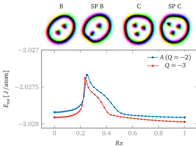
FIGURE 1.19 – Skyrmion colliding with the "sack" wall
