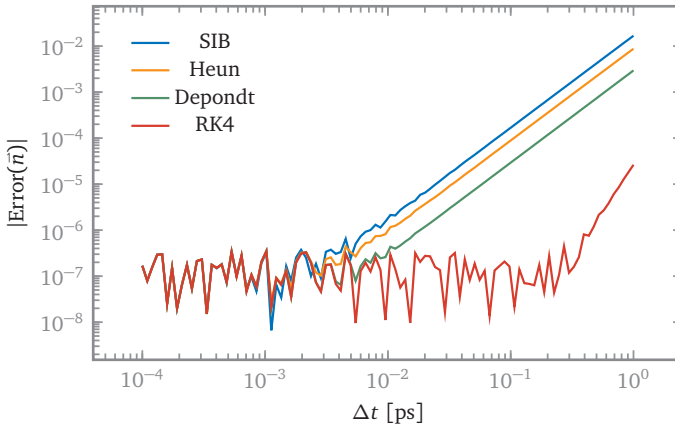
FIGURE 3.11 – Solvers' error dependence on time step
