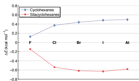
Figure 1. Conformational energies \Delta E = E_{ax} - E_{eq} for C_6H_{11}X and C_5H_{10}SiHX . 23 Copyright by the ACS Publications. Reproduced with permission.
