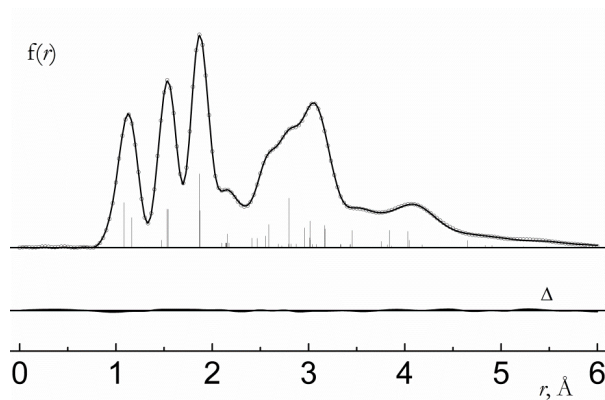
Figure 3. Experimental (dots) and calculated (solid lines) radial distribution curve for the axial conformer of 1-cyano-1-silacyclohexane 4 as obtained by gas electron diffraction. Below: difference curve (experiment – model).
