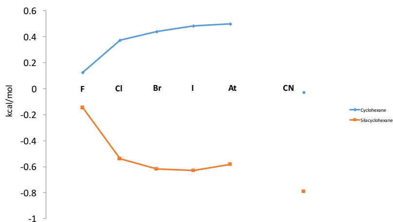
Figure 6. CCSD(T)/CBS computed axial/equatorial energy differences (kcal mol -1 ) of the halogen substituent series and the cyano group in both cyclohexane and silacyclohexane families. Modified from Figure 1 and reproduced with permission. 23
