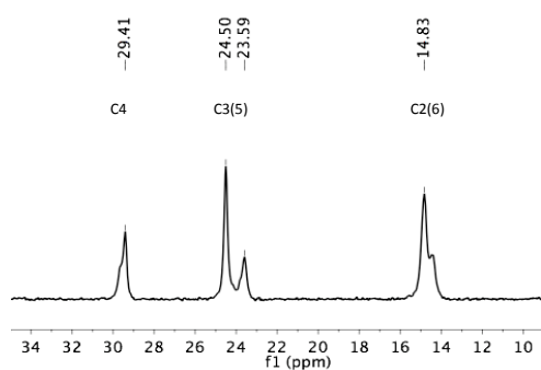
Figure 4. ^{13}\text{C} NMR spectrum of 1-cycano-1-sila-cyclohexane 4 at 110 K.
