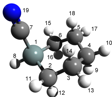
Figure 2. Molecular model and atom numbering of 1-cyano-1-silacyclohexane 4 (axial conformer).
