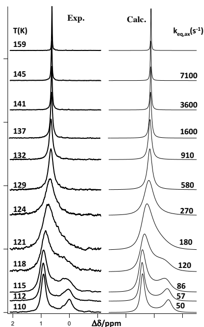
Figure 5. Low-temperature ^{13}\text{C} NMR spectra for the C3 and C5 atoms of 4 . Experimental spectra are to the left and simulated spectra are to the right.
